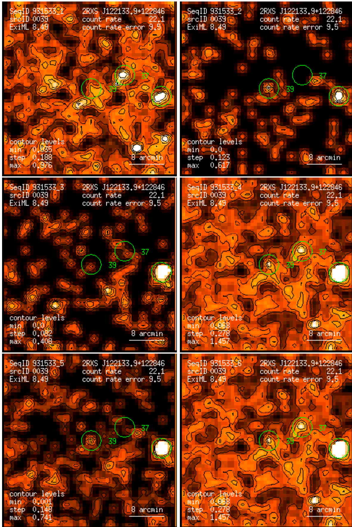
Figure 39: RASS 931533: detection 0039: band rate images, Gaussian filter: (1) PSPC channels 11 – 41, (2) 52 – 90, (3) 91 – 201, (4) 11 – 235, (5) 52 – 201, (6) 11 – 201. Broad band rates in counts/ks. Band rate contour levels in counts/ks/arcmin 2 .
