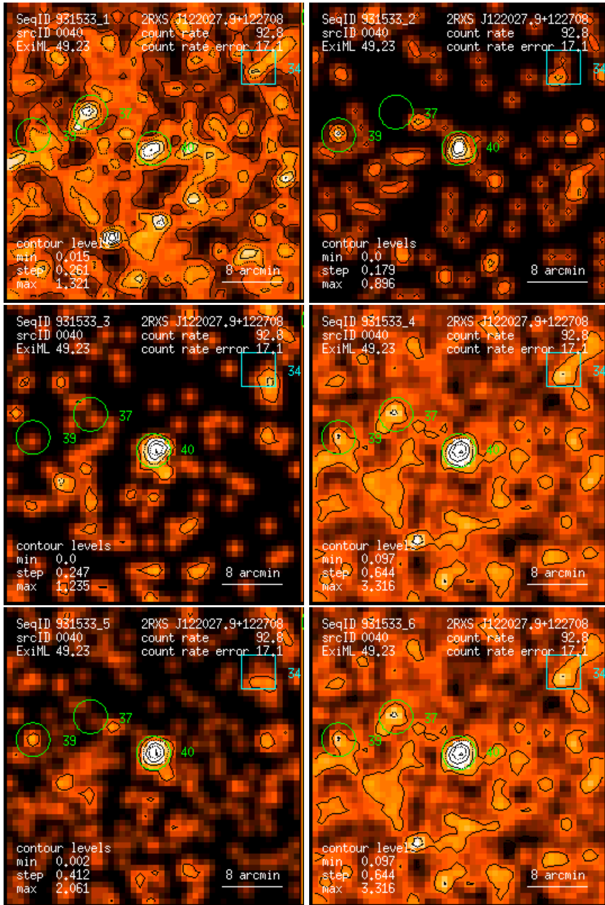
Figure 40: RASS 931533: detection 0040: band rate images, Gaussian filter: (1) PSPC channels 11 – 41, (2) 52 – 90, (3) 91 – 201, (4) 11 – 235, (5) 52 – 201, (6) 11 – 201. Broad band rates in counts/ks. Band rate contour levels in counts/ks/arcmin 2 .
