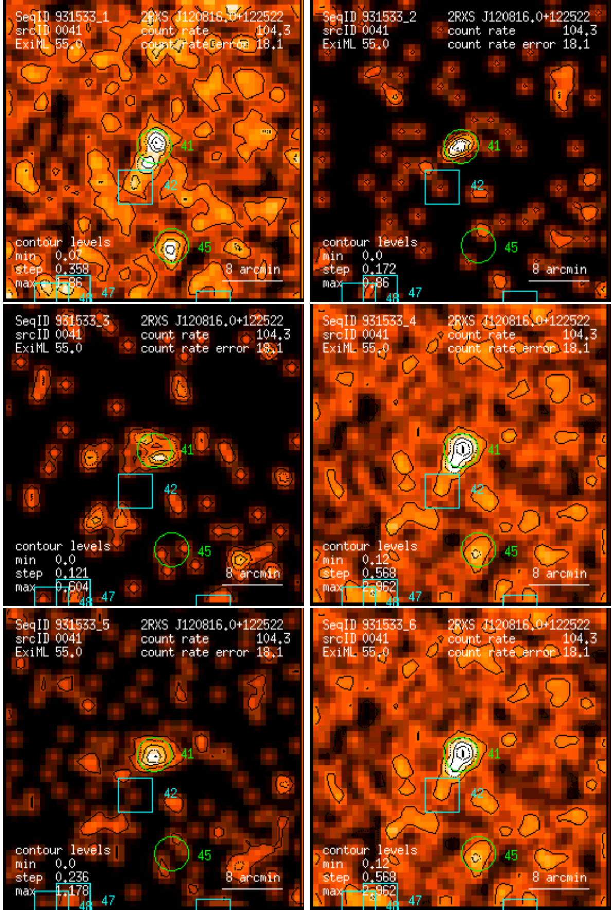
Figure 41: RASS 931533: detection 0041: band rate images, Gaussian filter: (1) PSPC channels 11 – 41, (2) 52 – 90, (3) 91 – 201, (4) 11 – 235, (5) 52 – 201, (6) 11 – 201. Broad band rates in counts/ks. Band rate contour levels in counts/ks/arcmin 2 .
