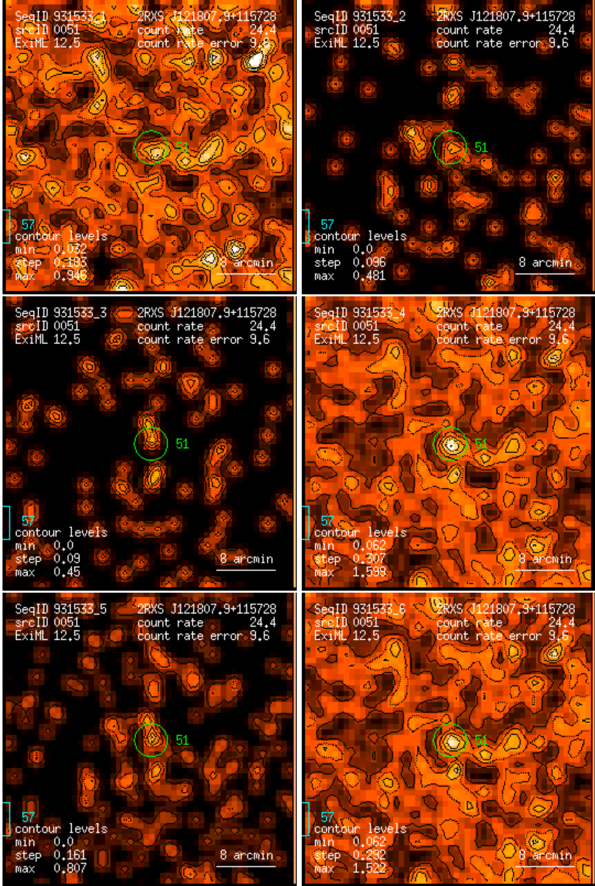
Figure 51: RASS 931533: detection 0051: band rate images, Gaussian filter: (1) PSPC channels 11 – 41, (2) 52 – 90, (3) 91 – 201, (4) 11 – 235, (5) 52 – 201, (6) 11 – 201. Broad band rates in counts/ks. Band rate contour levels in counts/ks/arcmin 2 .
