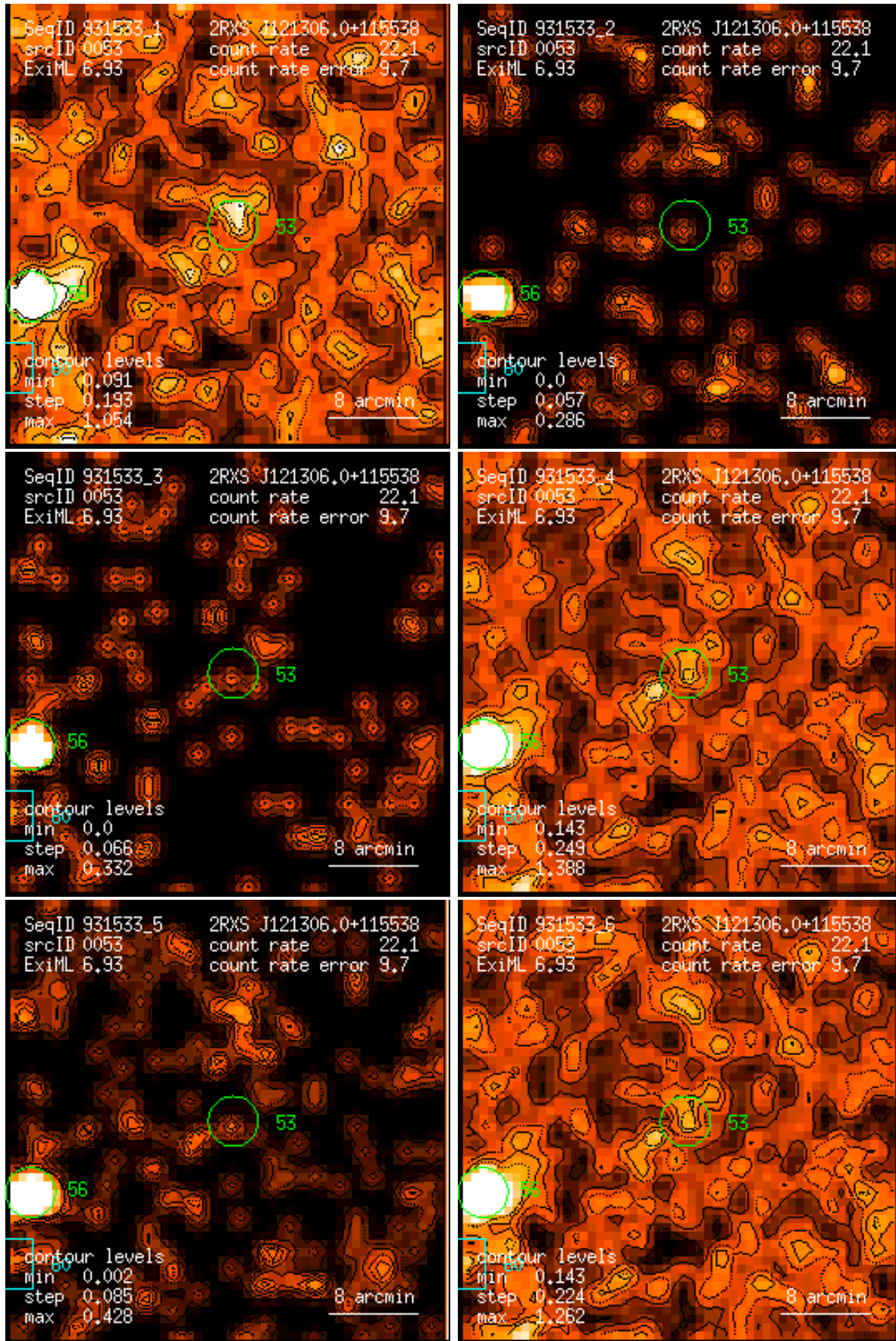
Figure 53: RASS 931533: detection 0053: band rate images, Gaussian filter: (1) PSPC channels 11 – 41, (2) 52 – 90, (3) 91 – 201, (4) 11 – 235, (5) 52 – 201, (6) 11 – 201. Broad band rates in counts/ks. Band rate contour levels in counts/ks/arcmin 2 .
