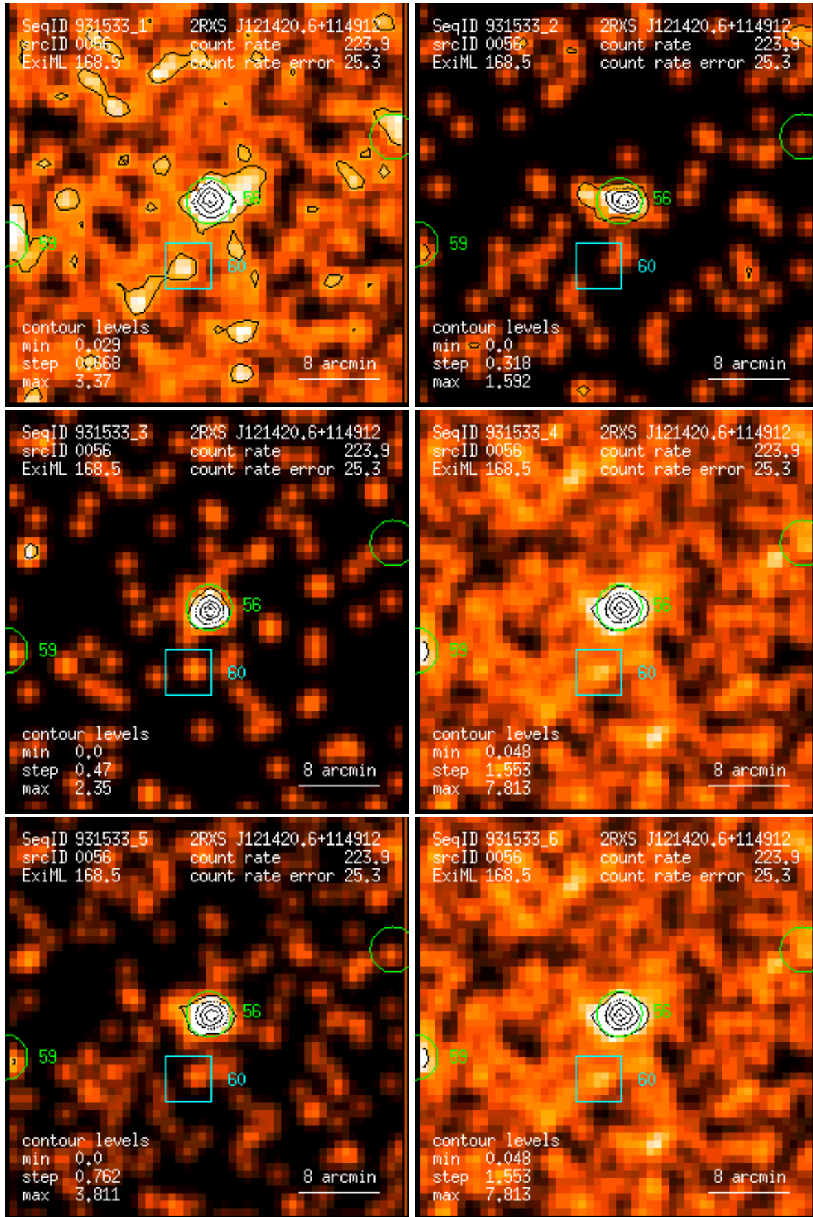
Figure 56: RASS 931533: detection 0056: band rate images, Gaussian filter: (1) PSPC channels 11 – 41, (2) 52 – 90, (3) 91 – 201, (4) 11 – 235, (5) 52 – 201, (6) 11 – 201. Broad band rates in counts/ks. Band rate contour levels in counts/ks/arcmin 2 .
