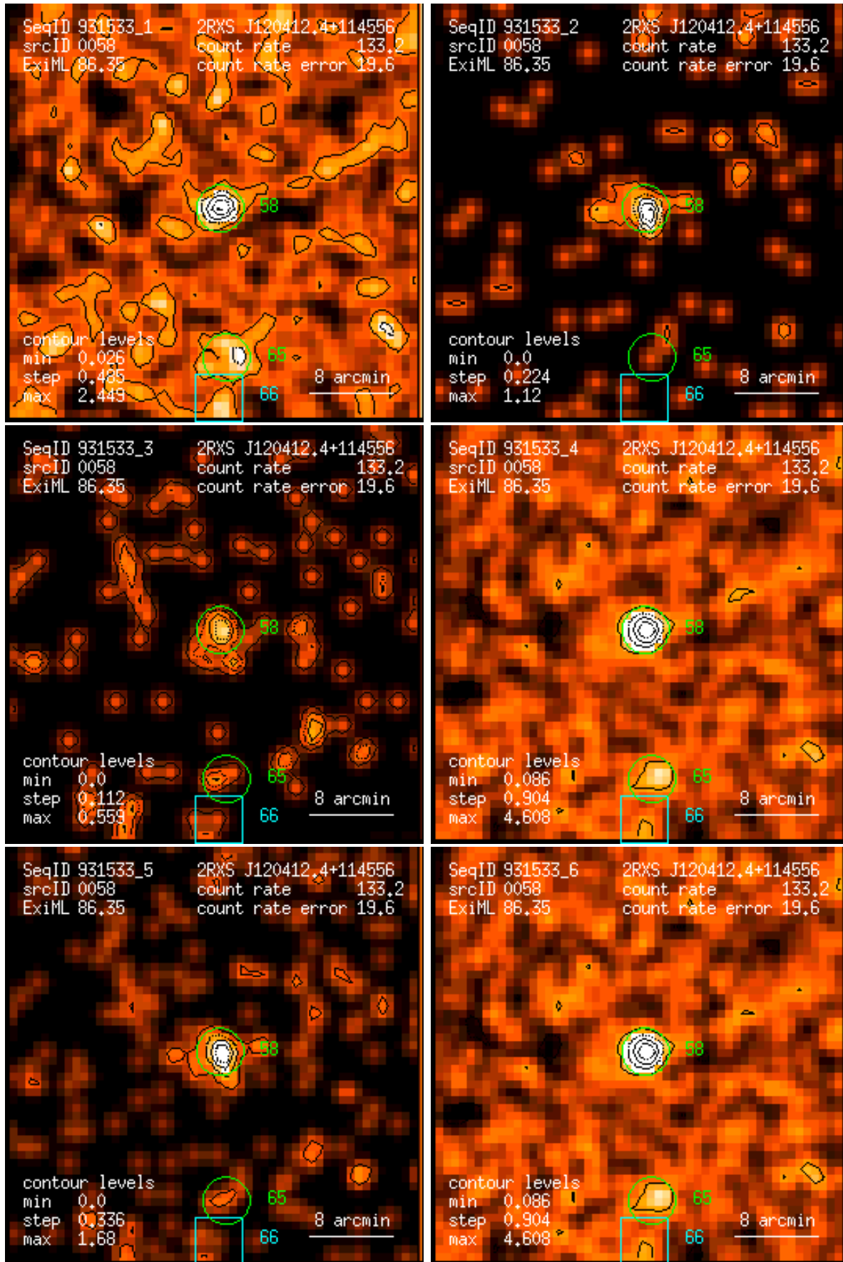
Figure 58: RASS 931533: detection 0058: band rate images, Gaussian filter: (1) PSPC channels 11 – 41, (2) 52 – 90, (3) 91 – 201, (4) 11 – 235, (5) 52 – 201, (6) 11 – 201. Broad band rates in counts/ks. Band rate contour levels in counts/ks/arcmin 2 .
