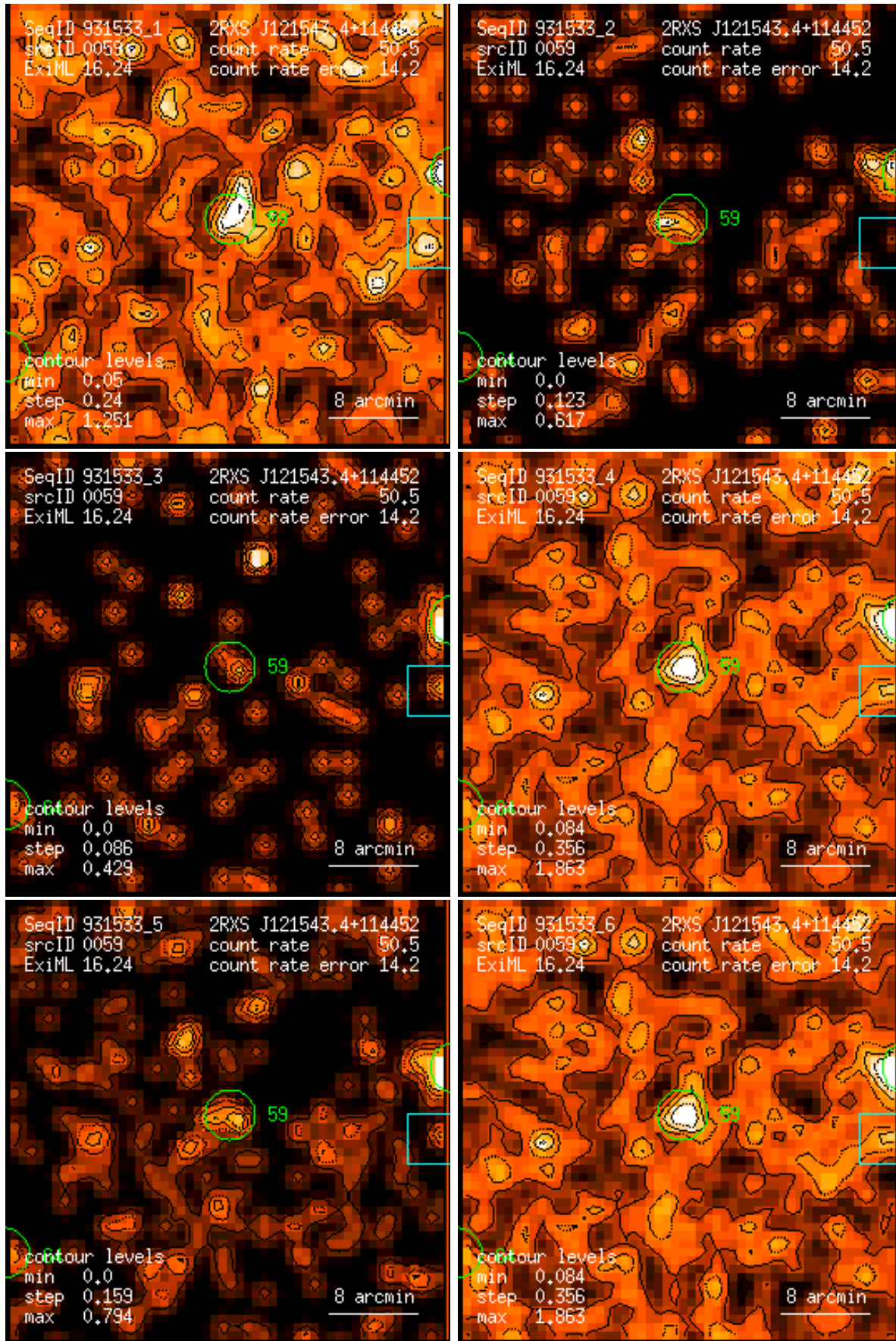
Figure 59: RASS 931533: detection 0059: band rate images, Gaussian filter: (1) PSPC channels 11 – 41, (2) 52 – 90, (3) 91 – 201, (4) 11 – 235, (5) 52 – 201, (6) 11 – 201. Broad band rates in counts/ks. Band rate contour levels in counts/ks/arcmin 2 .
