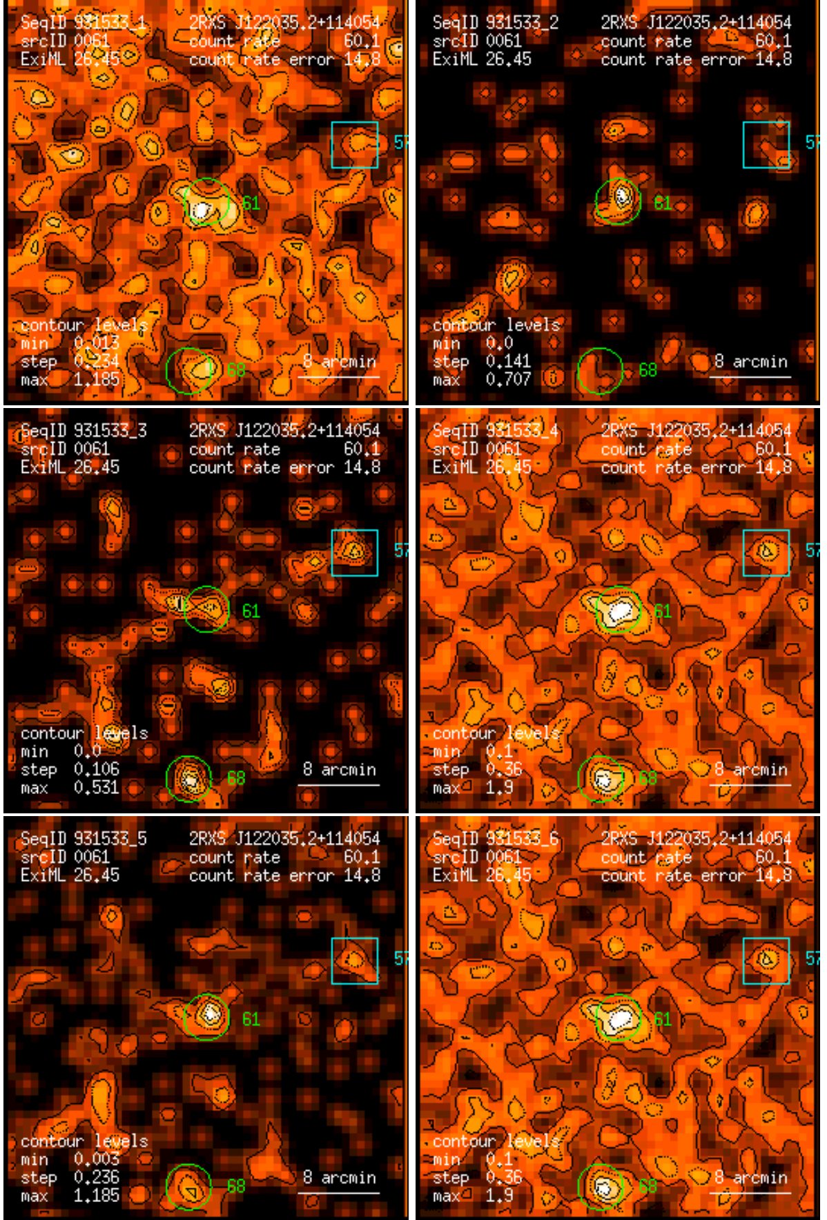
Figure 61: RASS 931533: detection 0061: band rate images, Gaussian filter: (1) PSPC channels 11 – 41, (2) 52 – 90, (3) 91 – 201, (4) 11 – 235, (5) 52 – 201, (6) 11 – 201. Broad band rates in counts/ks. Band rate contour levels in counts/ks/arcmin 2 .
