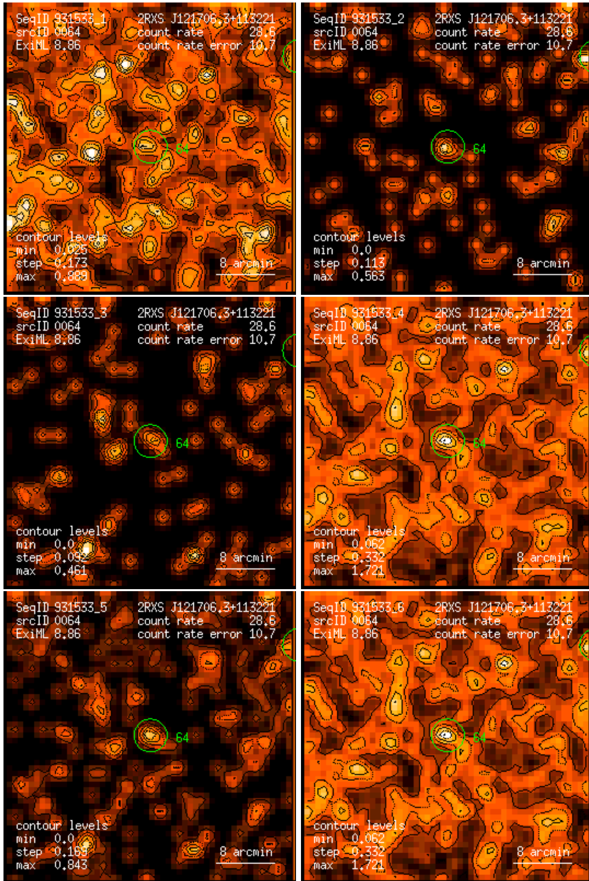
Figure 64: RASS 931533: detection 0064: band rate images, Gaussian filter: (1) PSPC channels 11 – 41, (2) 52 – 90, (3) 91 – 201, (4) 11 – 235, (5) 52 – 201, (6) 11 – 201. Broad band rates in counts/ks. Band rate contour levels in counts/ks/arcmin 2 .
