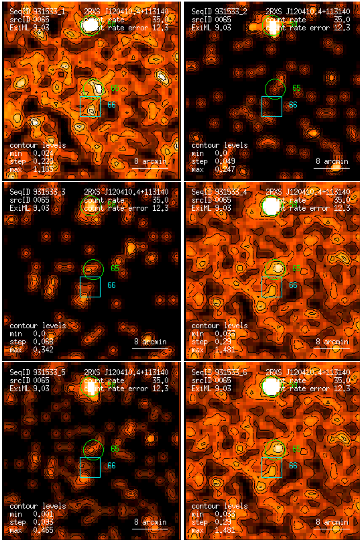
Figure 65: RASS 931533: detection 0065: band rate images, Gaussian filter: (1) PSPC channels 11 – 41, (2) 52 – 90, (3) 91 – 201, (4) 11 – 235, (5) 52 – 201, (6) 11 – 201. Broad band rates in counts/ks. Band rate contour levels in counts/ks/arcmin 2 .
