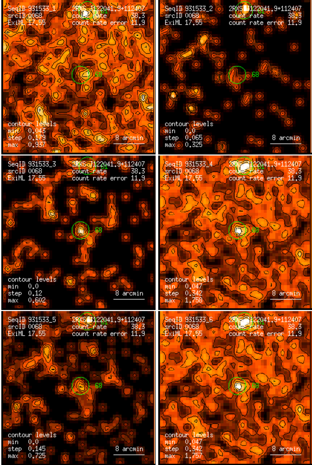
Figure 68: RASS 931533: detection 0068: band rate images, Gaussian filter: (1) PSPC channels 11 – 41, (2) 52 – 90, (3) 91 – 201, (4) 11 – 235, (5) 52 – 201, (6) 11 – 201. Broad band rates in counts/ks. Band rate contour levels in counts/ks/arcmin 2 .
