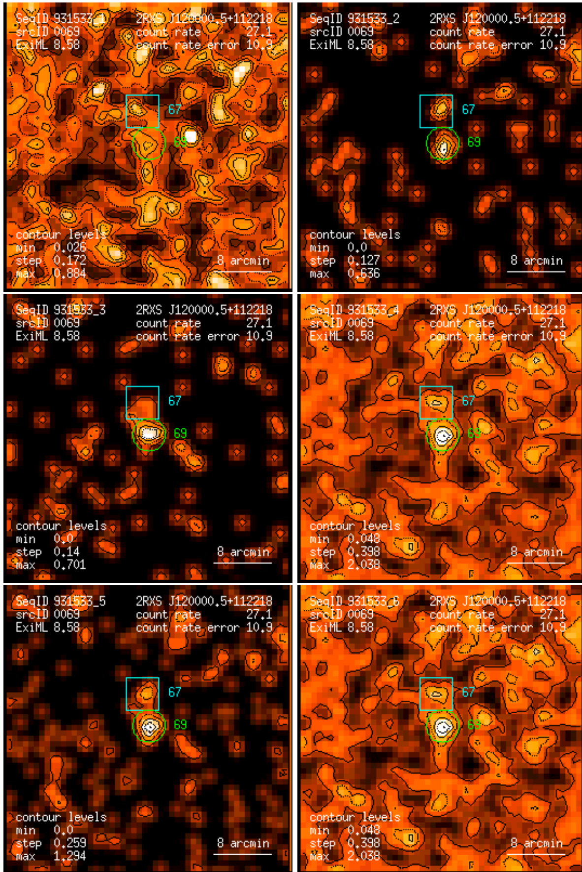
Figure 69: RASS 931533: detection 0069: band rate images, Gaussian filter: (1) PSPC channels 11 – 41, (2) 52 – 90, (3) 91 – 201, (4) 11 – 235, (5) 52 – 201, (6) 11 – 201. Broad band rates in counts/ks. Band rate contour levels in counts/ks/arcmin 2 .
