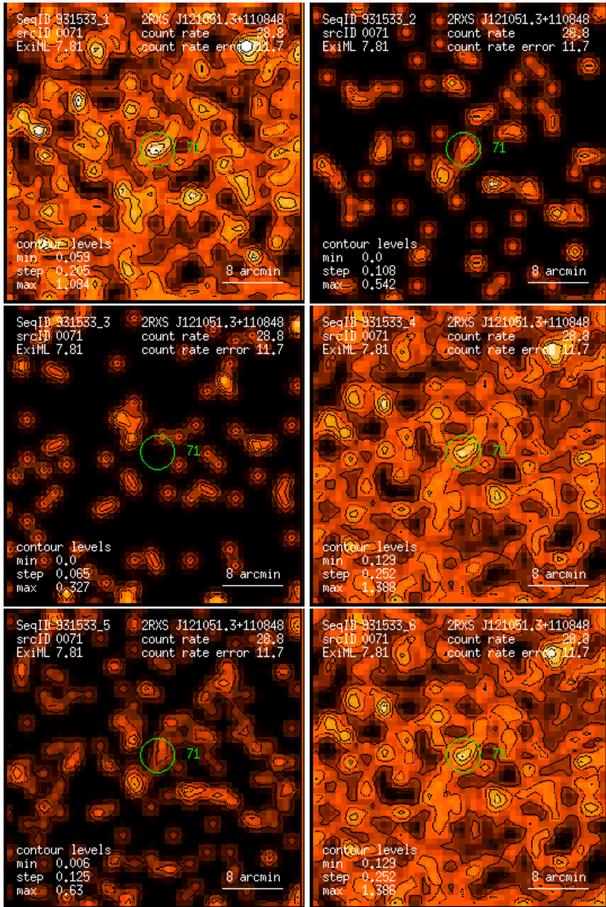
Figure 71: RASS 931533: detection 0071: band rate images, Gaussian filter: (1) PSPC channels 11 – 41, (2) 52 – 90, (3) 91 – 201, (4) 11 – 235, (5) 52 – 201, (6) 11 – 201. Broad band rates in counts/ks. Band rate contour levels in counts/ks/arcmin 2 .
