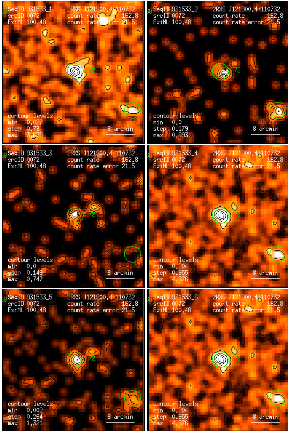
Figure 72: RASS 931533: detection 0072: band rate images, Gaussian filter: (1) PSPC channels 11 – 41, (2) 52 – 90, (3) 91 – 201, (4) 11 – 235, (5) 52 – 201, (6) 11 – 201. Broad band rates in counts/ks. Band rate contour levels in counts/ks/arcmin 2 .
