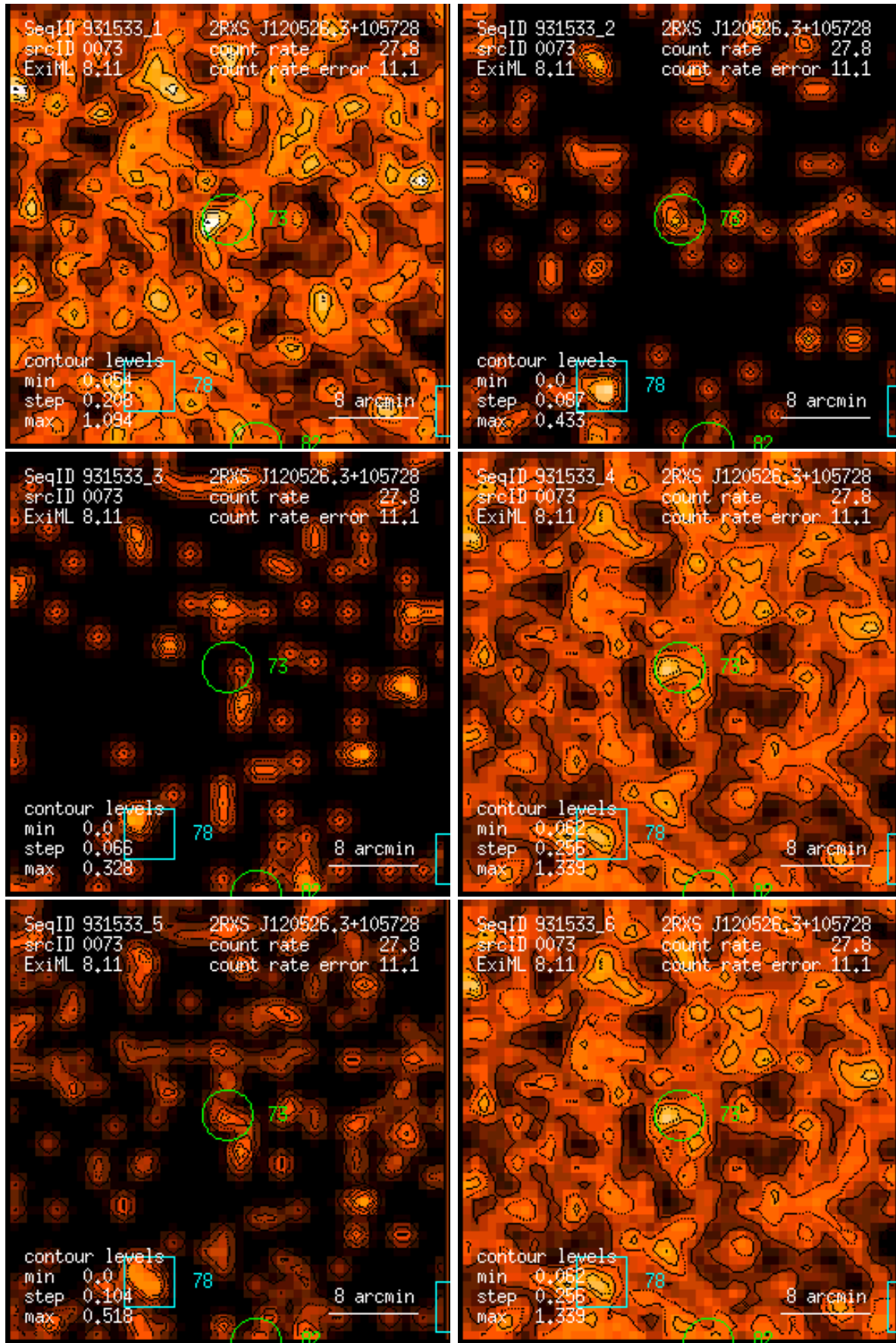
Figure 73: RASS 931533: detection 0073: band rate images, Gaussian filter: (1) PSPC channels 11 – 41, (2) 52 – 90, (3) 91 – 201, (4) 11 – 235, (5) 52 – 201, (6) 11 – 201. Broad band rates in counts/ks. Band rate contour levels in counts/ks/arcmin 2 .
