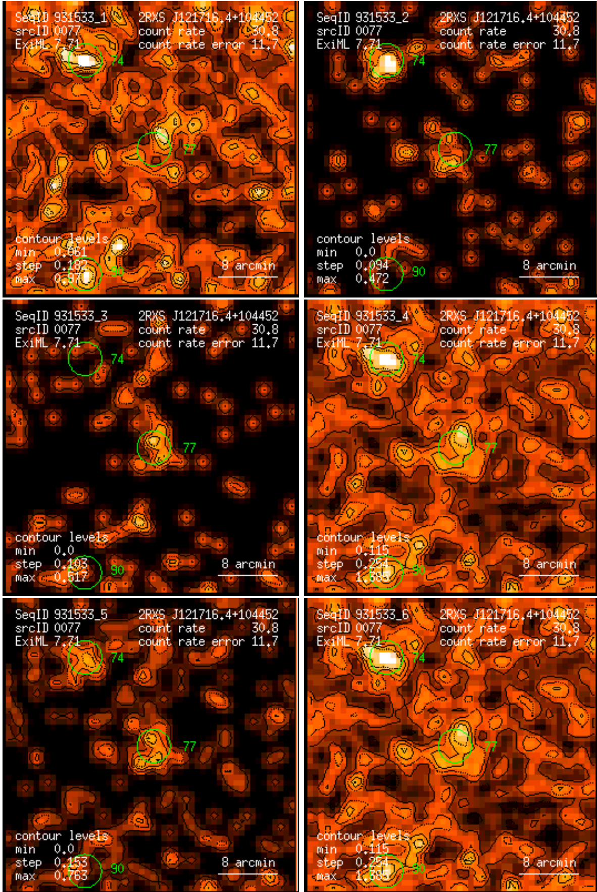
Figure 77: RASS 931533: detection 0077: band rate images, Gaussian filter: (1) PSPC channels 11 – 41, (2) 52 – 90, (3) 91 – 201, (4) 11 – 235, (5) 52 – 201, (6) 11 – 201. Broad band rates in counts/ks. Band rate contour levels in counts/ks/arcmin 2 .
