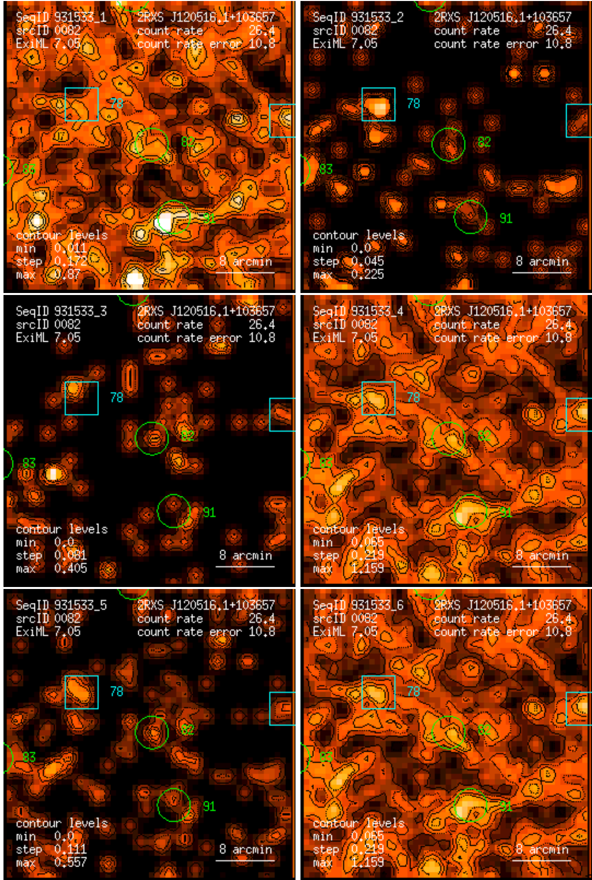
Figure 82: RASS 931533: detection 0082: band rate images, Gaussian filter: (1) PSPC channels 11 – 41, (2) 52 – 90, (3) 91 – 201, (4) 11 – 235, (5) 52 – 201, (6) 11 – 201. Broad band rates in counts/ks. Band rate contour levels in counts/ks/arcmin 2 .
