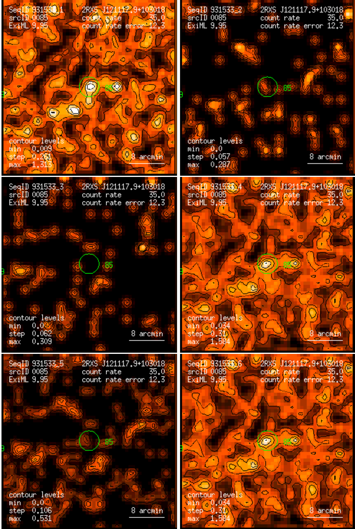
Figure 85: RASS 931533: detection 0085: band rate images, Gaussian filter: (1) PSPC channels 11 – 41, (2) 52 – 90, (3) 91 – 201, (4) 11 – 235, (5) 52 – 201, (6) 11 – 201. Broad band rates in counts/ks. Band rate contour levels in counts/ks/arcmin 2 .
