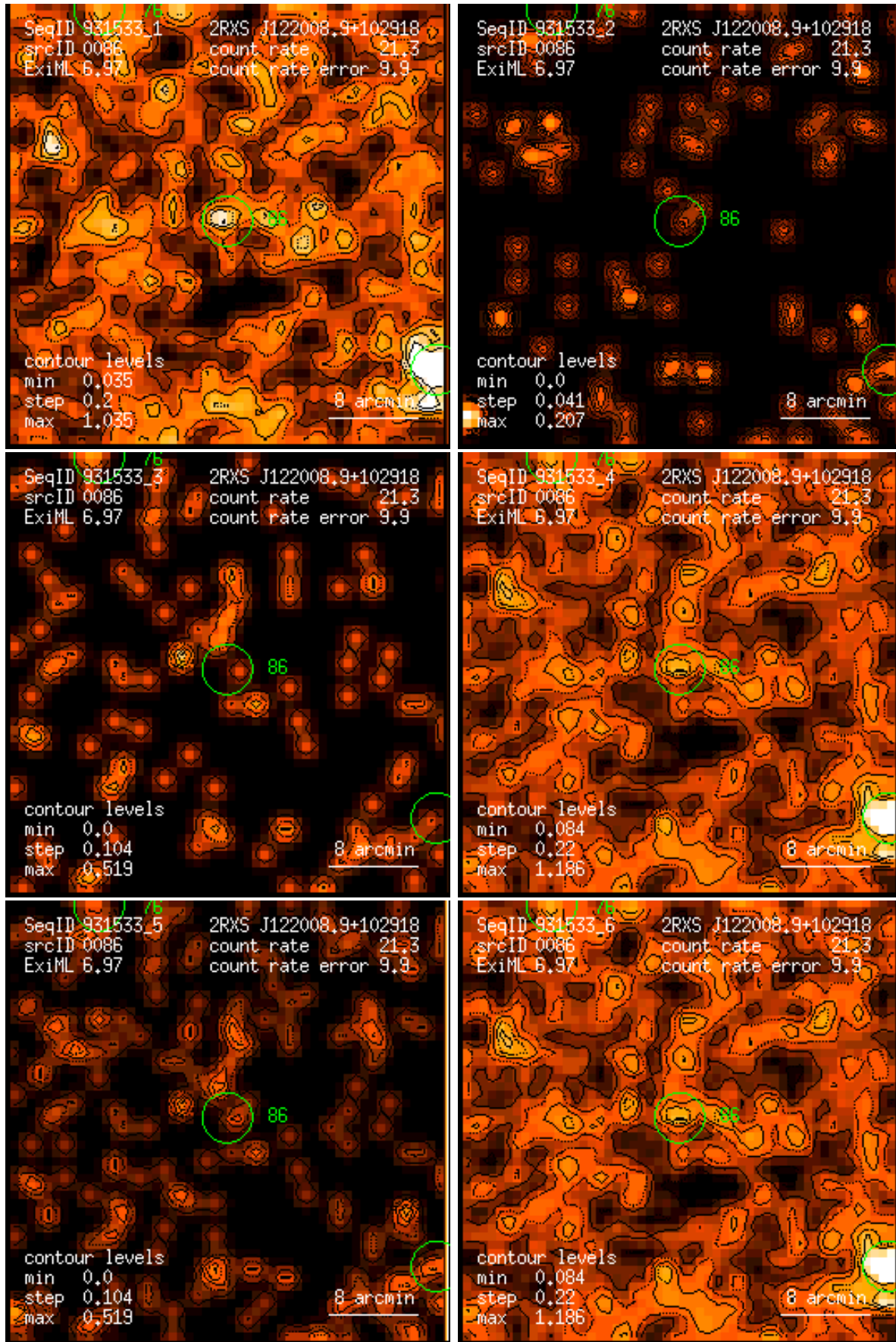
Figure 86: RASS 931533: detection 0086: band rate images, Gaussian filter: (1) PSPC channels 11 – 41, (2) 52 – 90, (3) 91 – 201, (4) 11 – 235, (5) 52 – 201, (6) 11 – 201. Broad band rates in counts/ks. Band rate contour levels in counts/ks/arcmin 2 .
