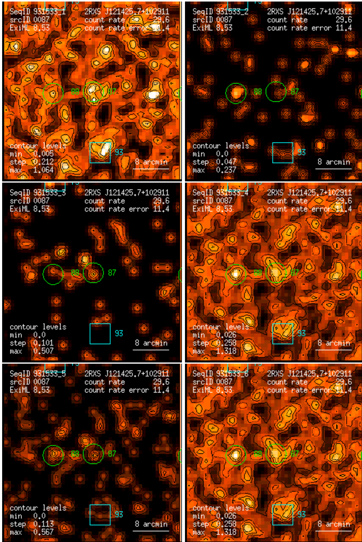
Figure 87: RASS 931533: detection 0087: band rate images, Gaussian filter: (1) PSPC channels 11 – 41, (2) 52 – 90, (3) 91 – 201, (4) 11 – 235, (5) 52 – 201, (6) 11 – 201. Broad band rates in counts/ks. Band rate contour levels in counts/ks/arcmin 2 .
