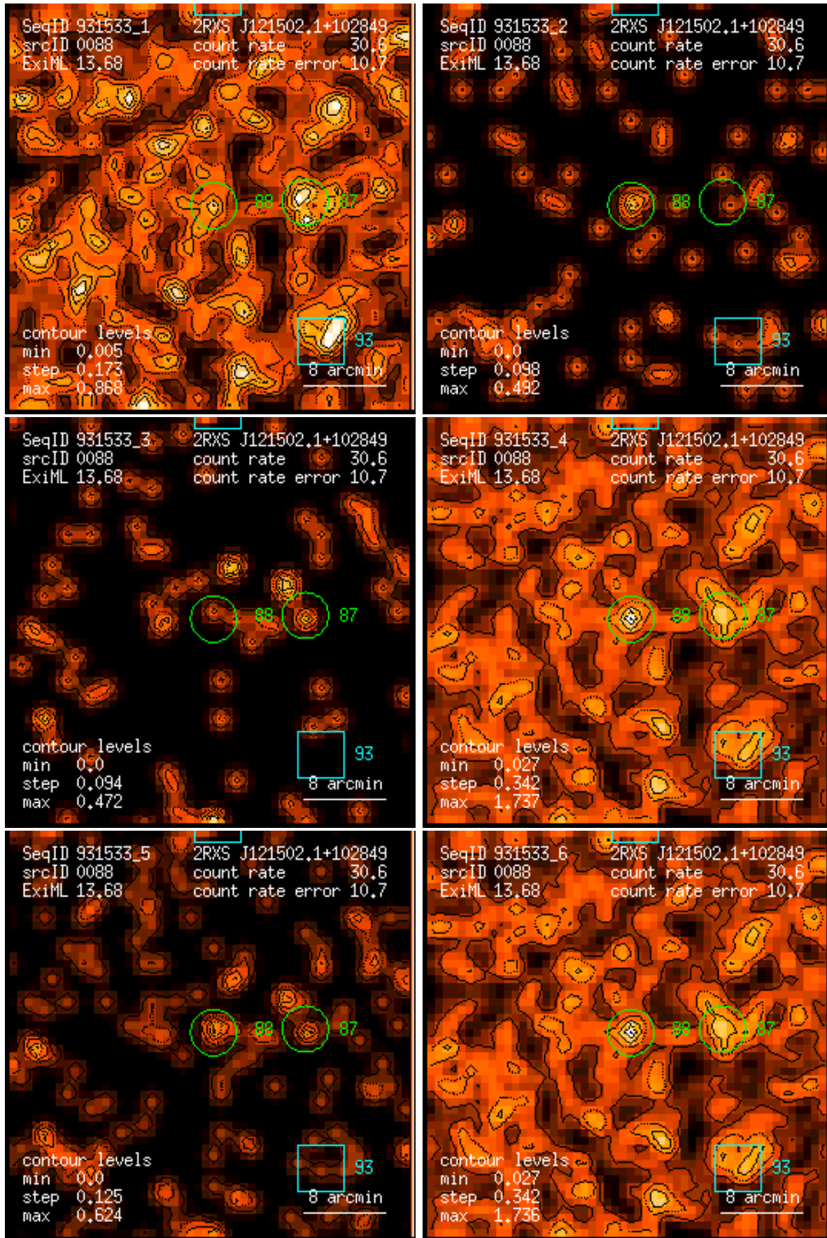
Figure 88: RASS 931533: detection 0088: band rate images, Gaussian filter: (1) PSPC channels 11 – 41, (2) 52 – 90, (3) 91 – 201, (4) 11 – 235, (5) 52 – 201, (6) 11 – 201. Broad band rates in counts/ks. Band rate contour levels in counts/ks/arcmin 2 .
