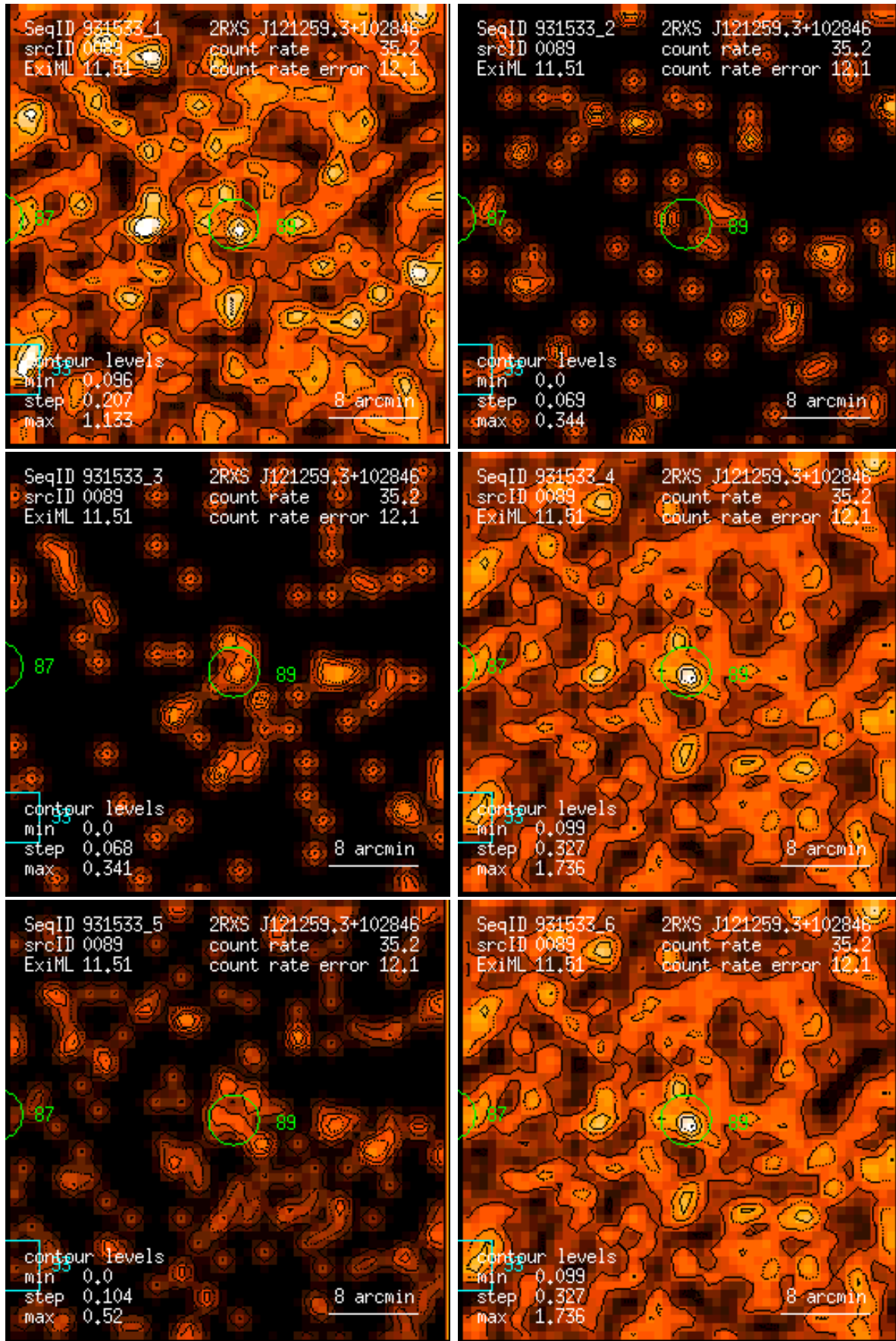
Figure 89: RASS 931533: detection 0089: band rate images, Gaussian filter: (1) PSPC channels 11 – 41, (2) 52 – 90, (3) 91 – 201, (4) 11 – 235, (5) 52 – 201, (6) 11 – 201. Broad band rates in counts/ks. Band rate contour levels in counts/ks/arcmin 2 .
