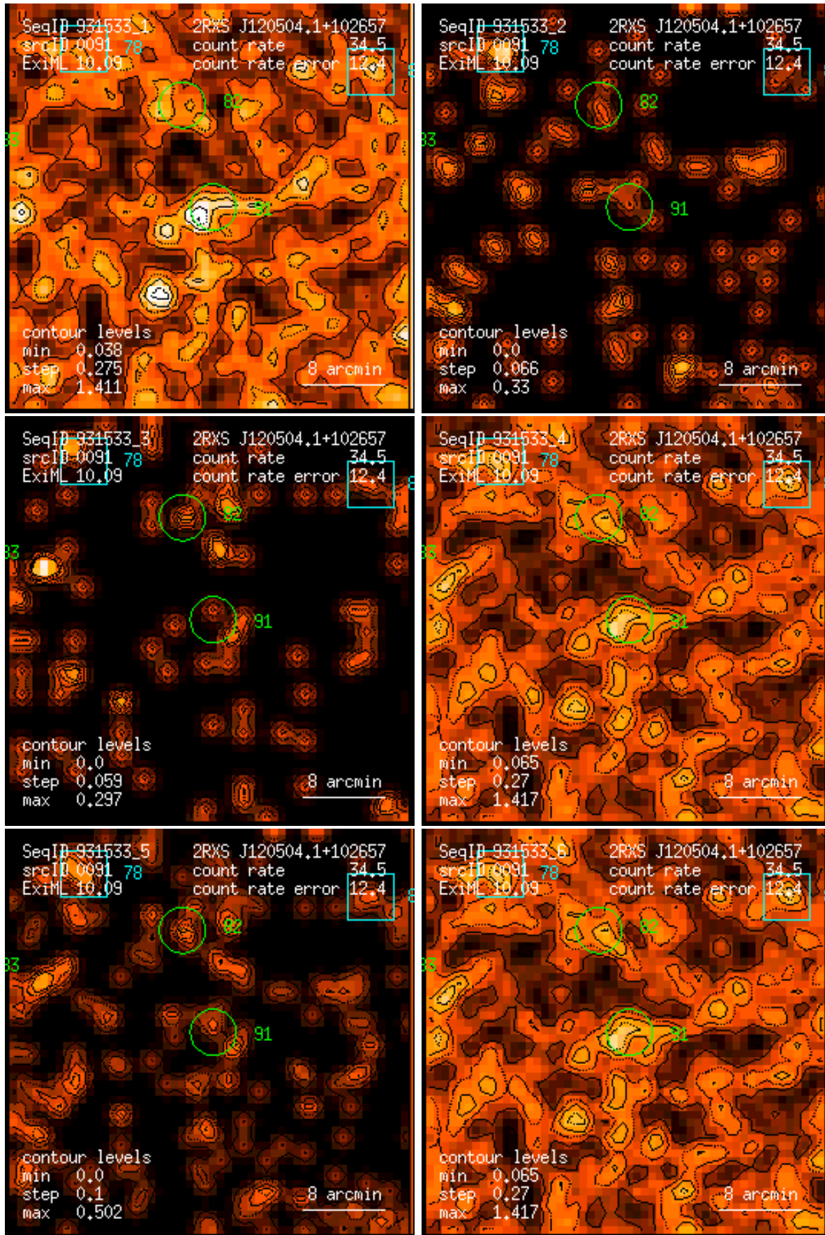
Figure 91: RASS 931533: detection 0091: band rate images, Gaussian filter: (1) PSPC channels 11 – 41, (2) 52 – 90, (3) 91 – 201, (4) 11 – 235, (5) 52 – 201, (6) 11 – 201. Broad band rates in counts/ks. Band rate contour levels in counts/ks/arcmin 2 .
