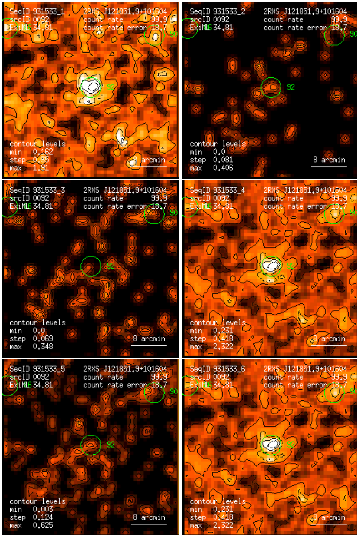
Figure 92: RASS 931533: detection 0092: band rate images, Gaussian filter: (1) PSPC channels 11 – 41, (2) 52 – 90, (3) 91 – 201, (4) 11 – 235, (5) 52 – 201, (6) 11 – 201. Broad band rates in counts/ks. Band rate contour levels in counts/ks/arcmin 2 .
