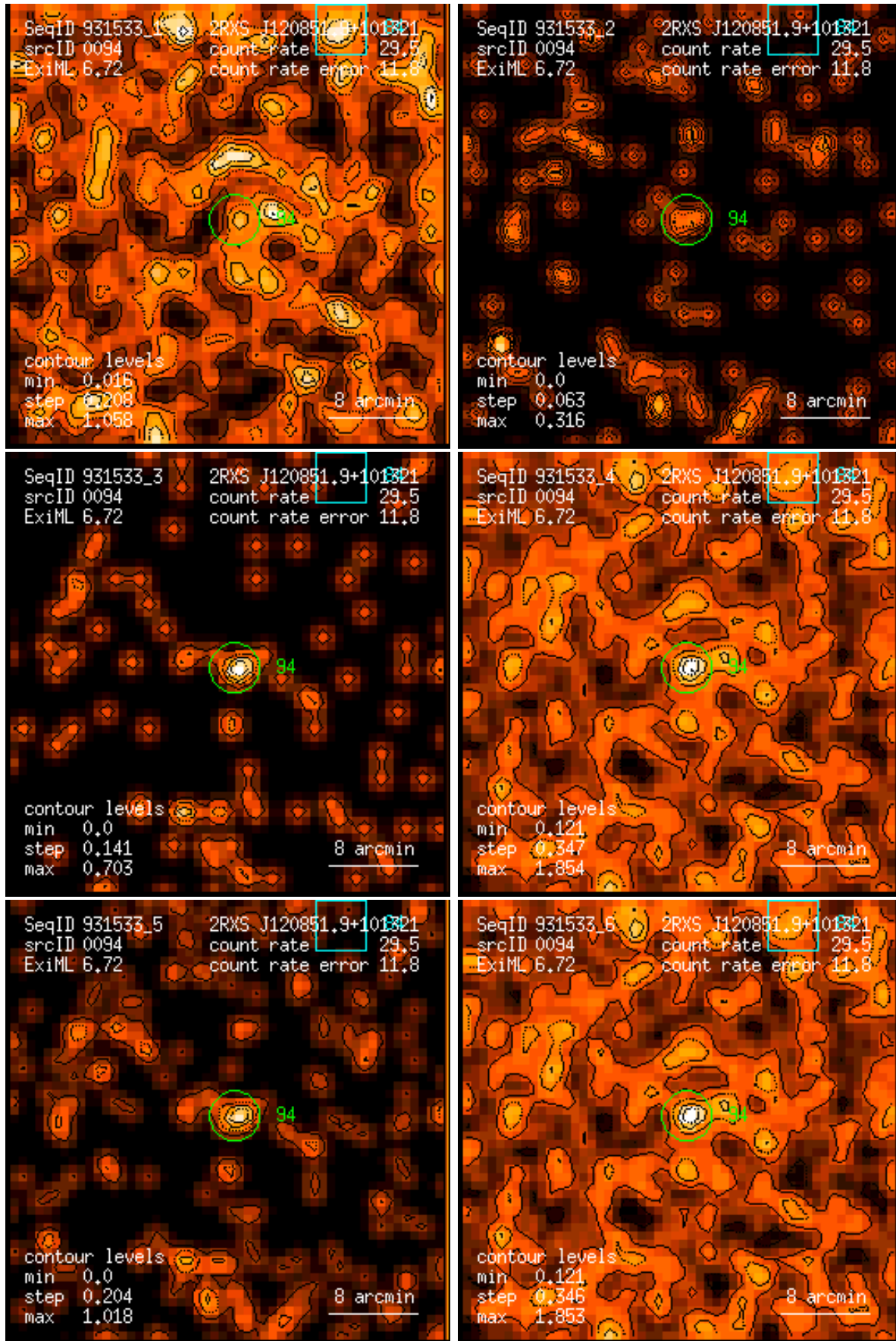
Figure 94: RASS 931533: detection 0094: band rate images, Gaussian filter: (1) PSPC channels 11 – 41, (2) 52 – 90, (3) 91 – 201, (4) 11 – 235, (5) 52 – 201, (6) 11 – 201. Broad band rates in counts/ks. Band rate contour levels in counts/ks/arcmin 2 .
