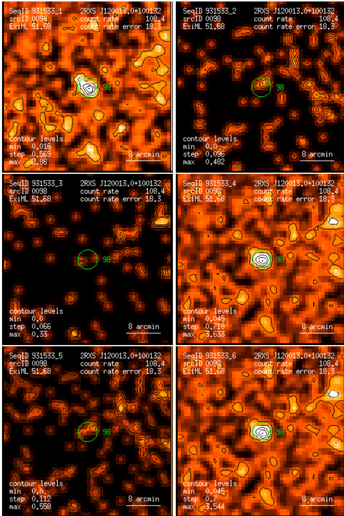
Figure 98: RASS 931533: detection 0098: band rate images, Gaussian filter: (1) PSPC channels 11 – 41, (2) 52 – 90, (3) 91 – 201, (4) 11 – 235, (5) 52 – 201, (6) 11 – 201. Broad band rates in counts/ks. Band rate contour levels in counts/ks/arcmin 2 .
