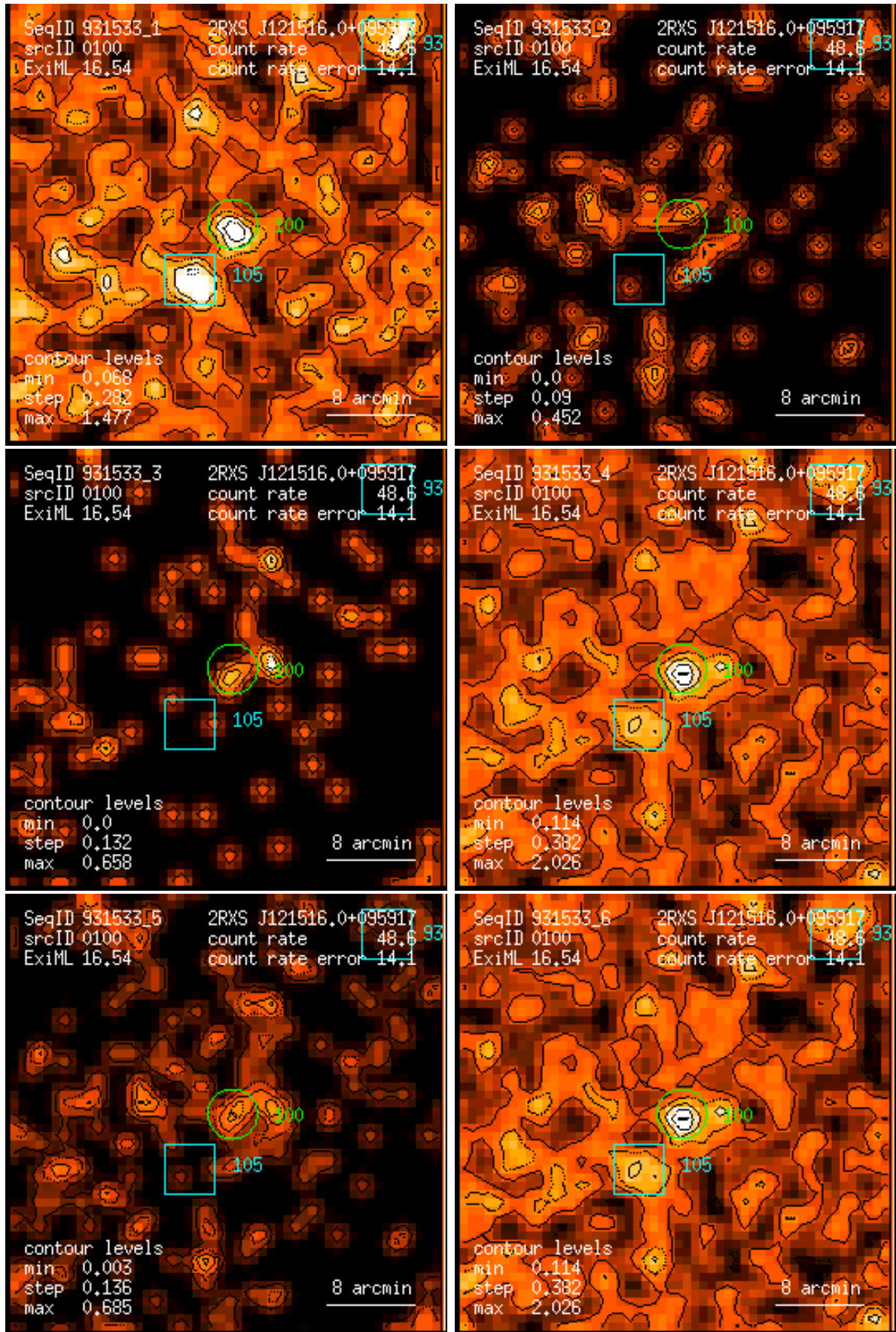
Figure 100: RASS 931533: detection 0100: band rate images, Gaussian filter: (1) PSPC channels 11 – 41, (2) 52 – 90, (3) 91 – 201, (4) 11 – 235, (5) 52 – 201, (6) 11 – 201. Broad band rates in counts/ks. Band rate contour levels in counts/ks/arcmin 2 .
