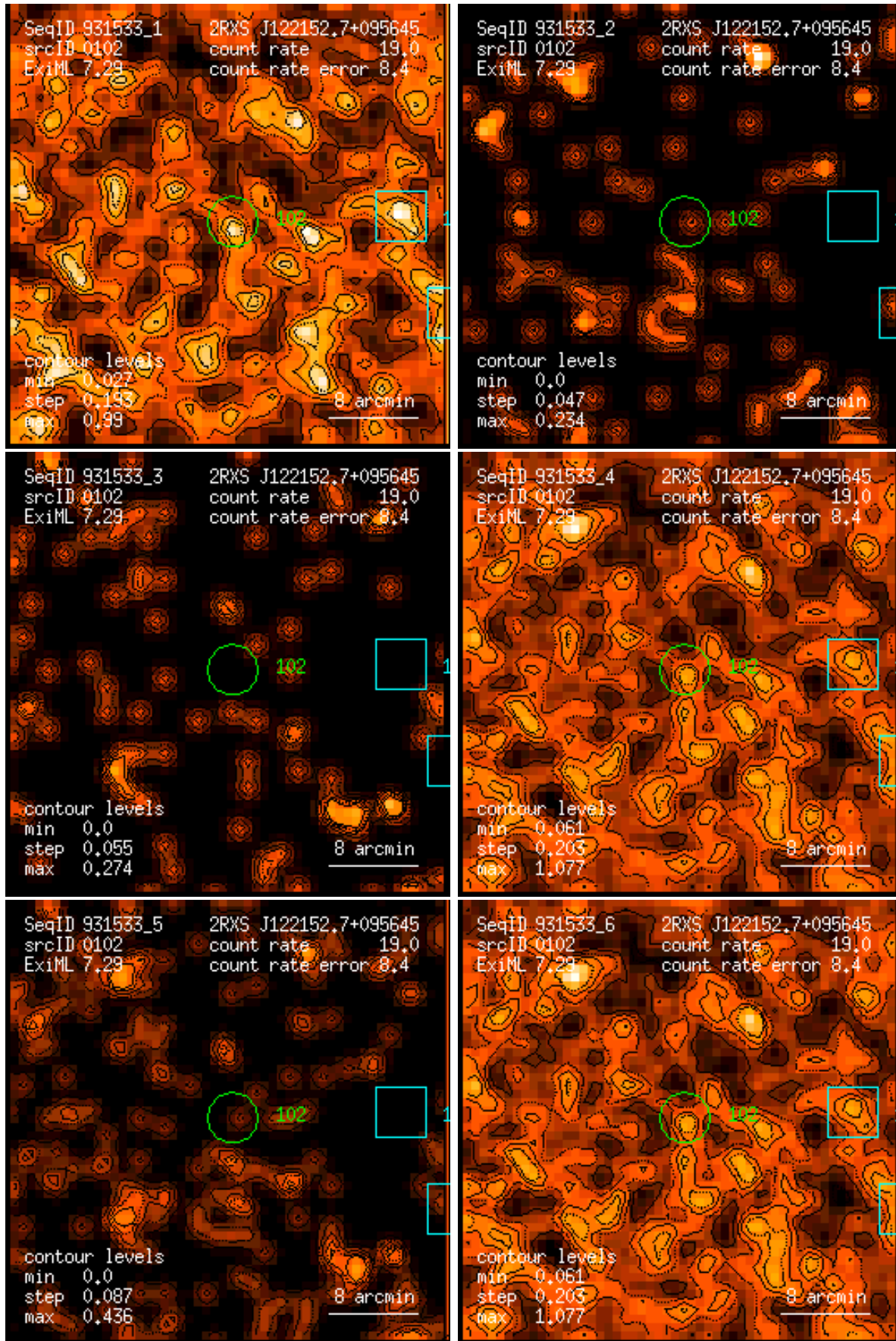
Figure 102: RASS 931533: detection 0102: band rate images, Gaussian filter: (1) PSPC channels 11 – 41, (2) 52 – 90, (3) 91 – 201, (4) 11 – 235, (5) 52 – 201, (6) 11 – 201. Broad band rates in counts/ks. Band rate contour levels in counts/ks/arcmin 2 .
