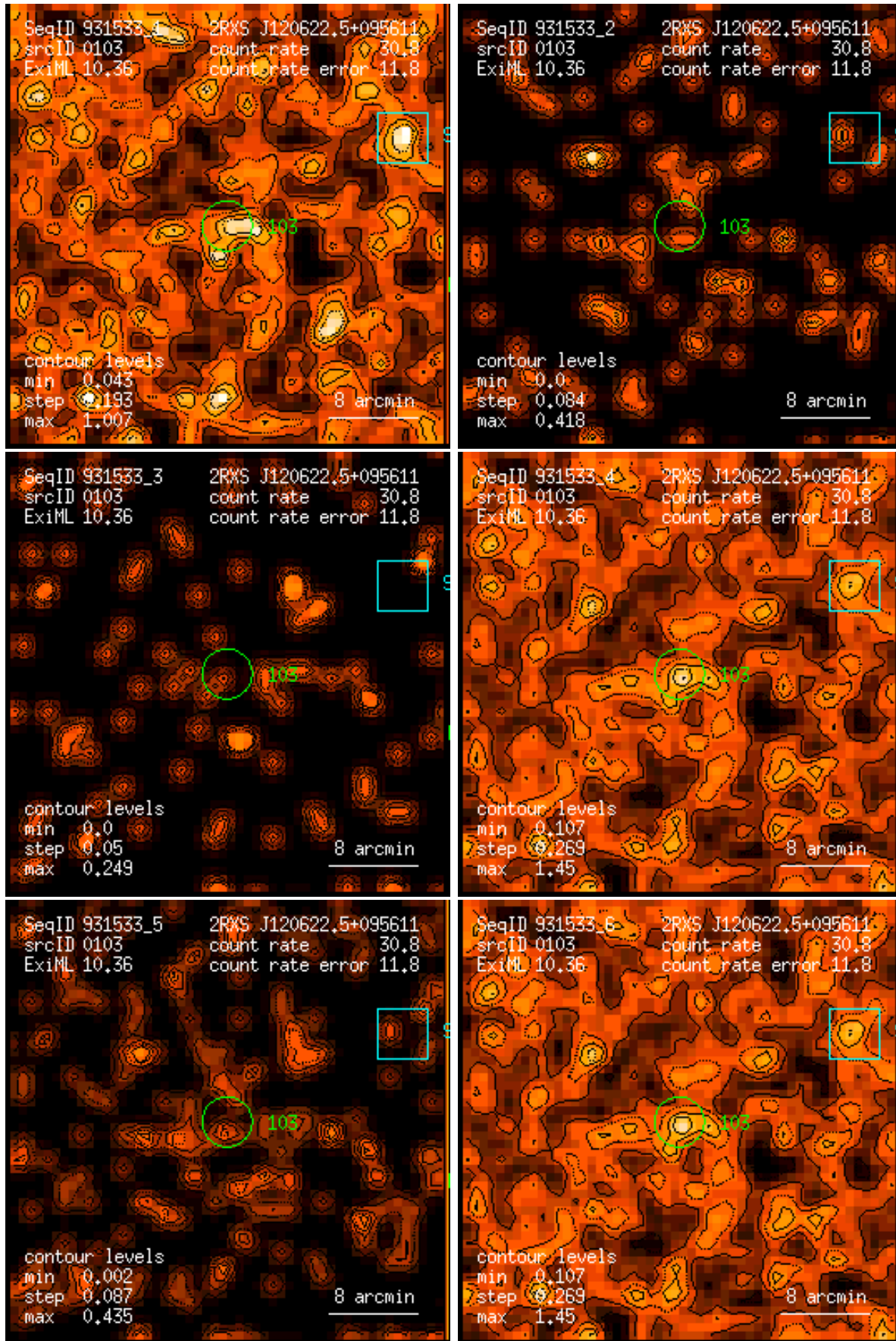
Figure 103: RASS 931533: detection 0103: band rate images, Gaussian filter: (1) PSPC channels 11 – 41, (2) 52 – 90, (3) 91 – 201, (4) 11 – 235, (5) 52 – 201, (6) 11 – 201. Broad band rates in counts/ks. Band rate contour levels in counts/ks/arcmin 2 .
