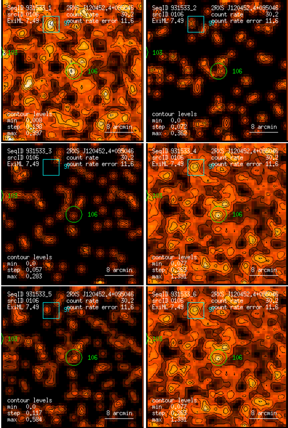
Figure 106: RASS 931533: detection 0106: band rate images, Gaussian filter: (1) PSPC channels 11 – 41, (2) 52 – 90, (3) 91 – 201, (4) 11 – 235, (5) 52 – 201, (6) 11 – 201. Broad band rates in counts/ks. Band rate contour levels in counts/ks/arcmin 2 .
