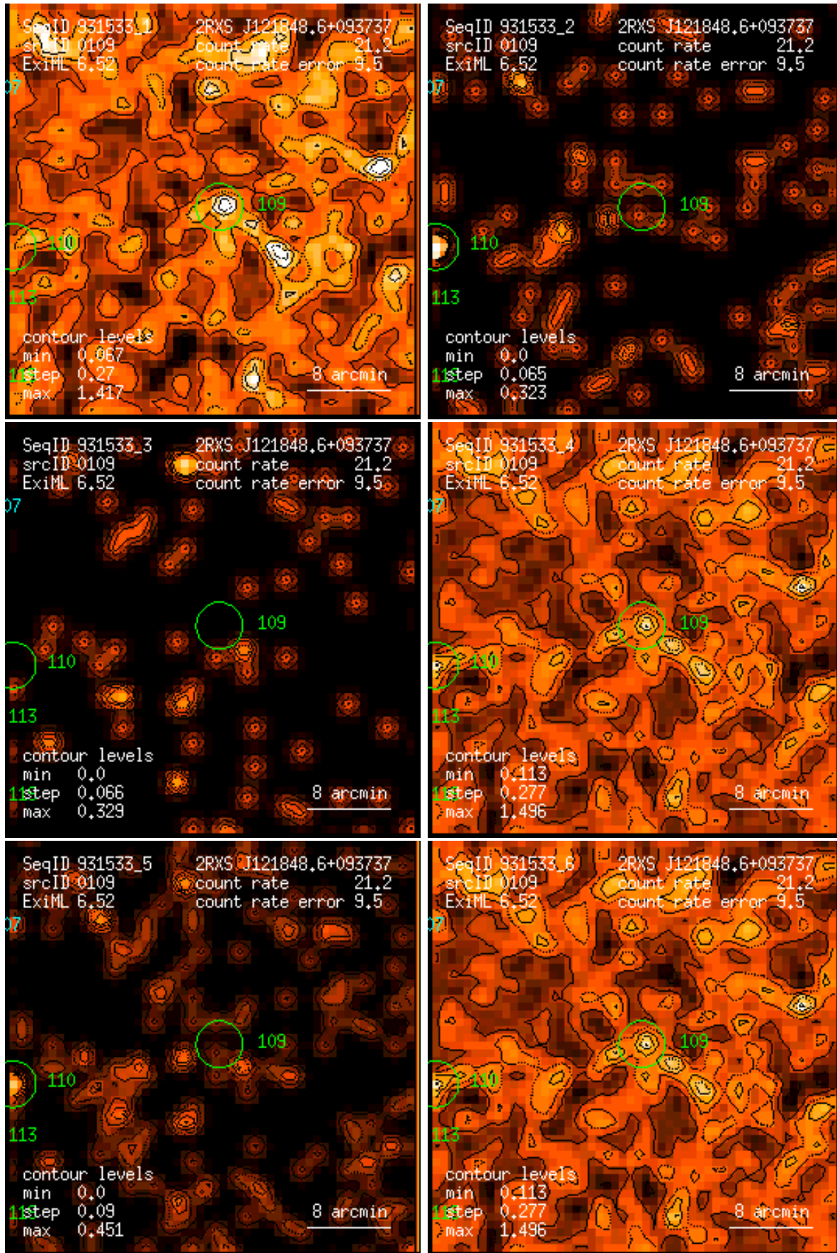
Figure 109: RASS 931533: detection 0109: band rate images, Gaussian filter: (1) PSPC channels 11 – 41, (2) 52 – 90, (3) 91 – 201, (4) 11 – 235, (5) 52 – 201, (6) 11 – 201. Broad band rates in counts/ks. Band rate contour levels in counts/ks/arcmin 2 .
