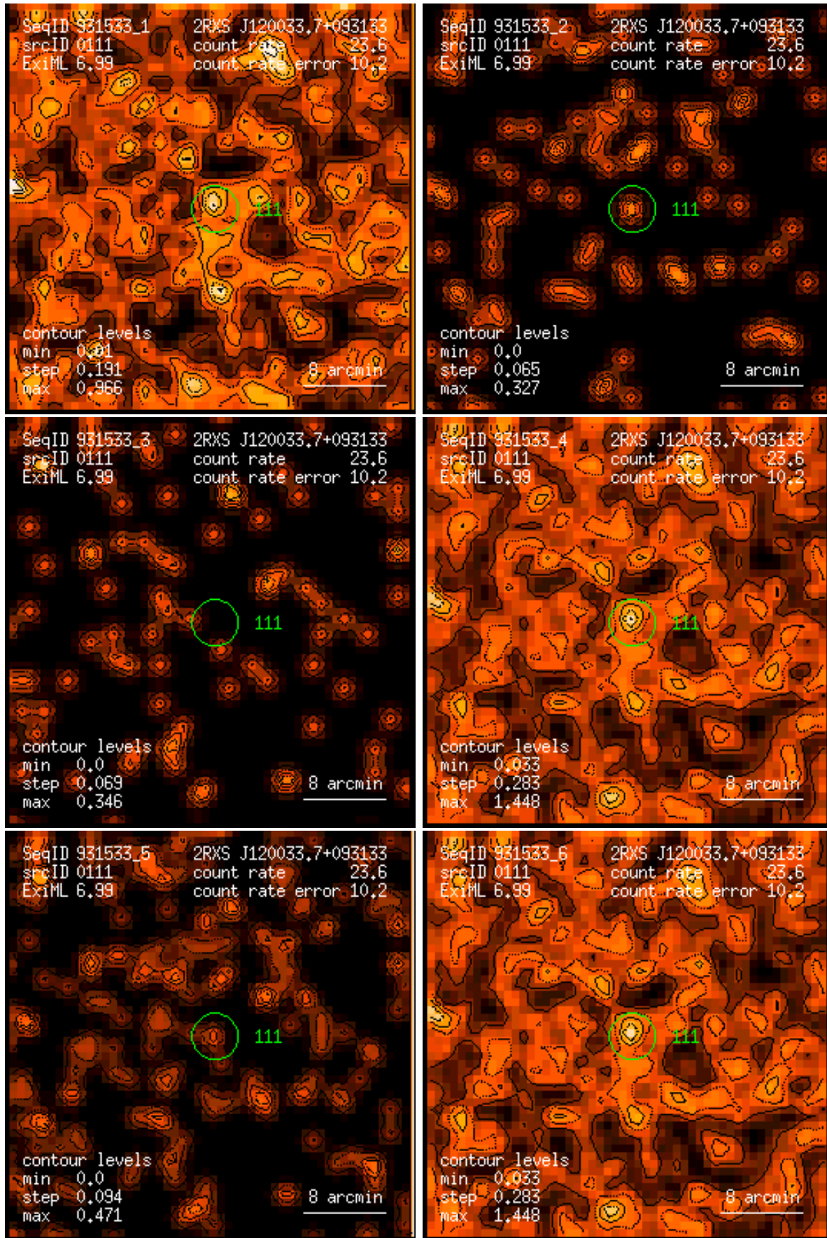
Figure 111: RASS 931533: detection 0111: band rate images, Gaussian filter: (1) PSPC channels 11 – 41, (2) 52 – 90, (3) 91 – 201, (4) 11 – 235, (5) 52 – 201, (6) 11 – 201. Broad band rates in counts/ks. Band rate contour levels in counts/ks/arcmin 2 .
