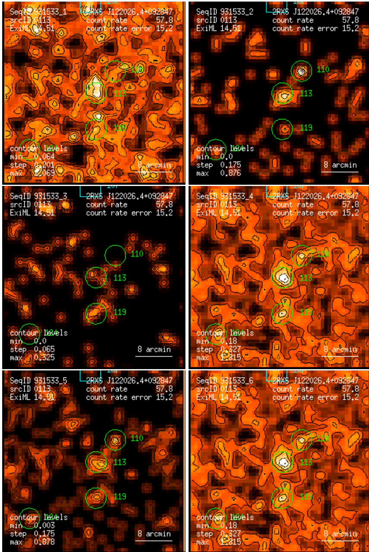
Figure 113: RASS 931533: detection 0113: band rate images, Gaussian filter: (1) PSPC channels 11 – 41, (2) 52 – 90, (3) 91 – 201, (4) 11 – 235, (5) 52 – 201, (6) 11 – 201. Broad band rates in counts/ks. Band rate contour levels in counts/ks/arcmin 2 .
