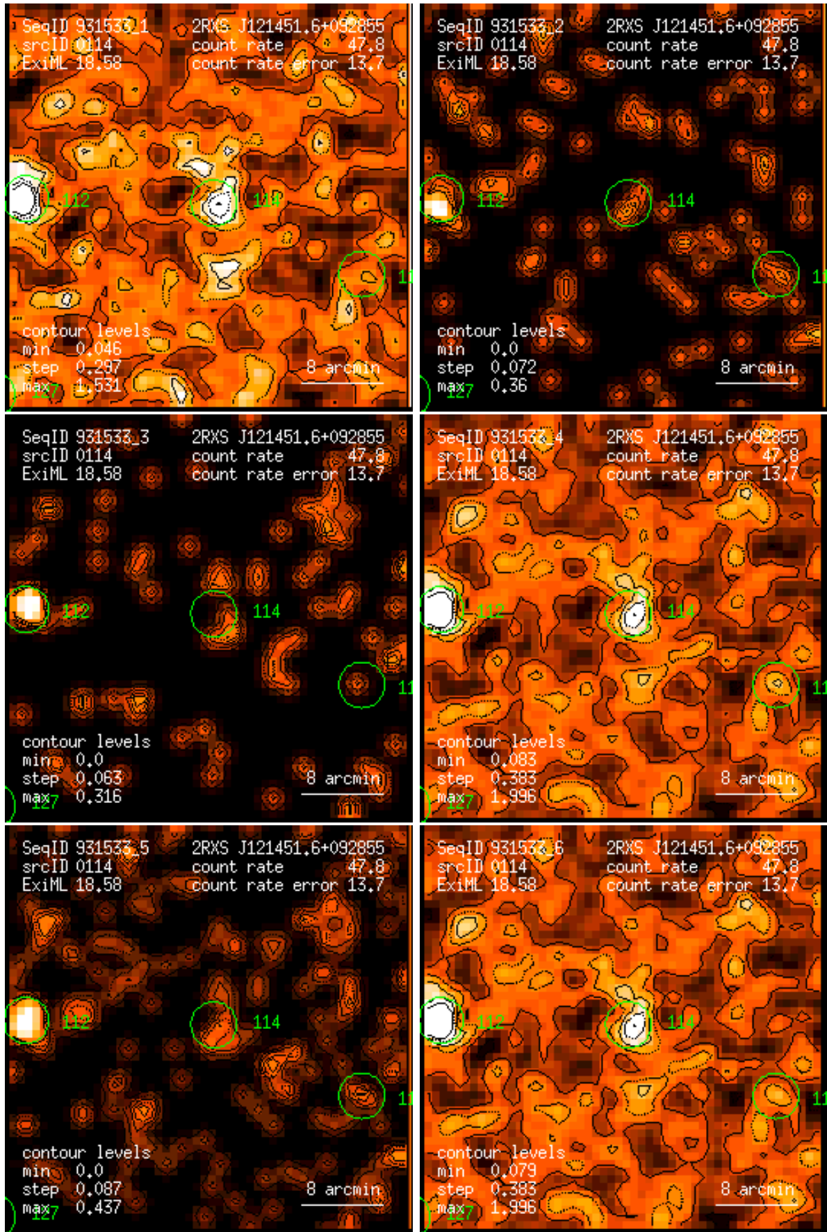
Figure 114: RASS 931533: detection 0114: band rate images, Gaussian filter: (1) PSPC channels 11 – 41, (2) 52 – 90, (3) 91 – 201, (4) 11 – 235, (5) 52 – 201, (6) 11 – 201. Broad band rates in counts/ks. Band rate contour levels in counts/ks/arcmin 2 .
