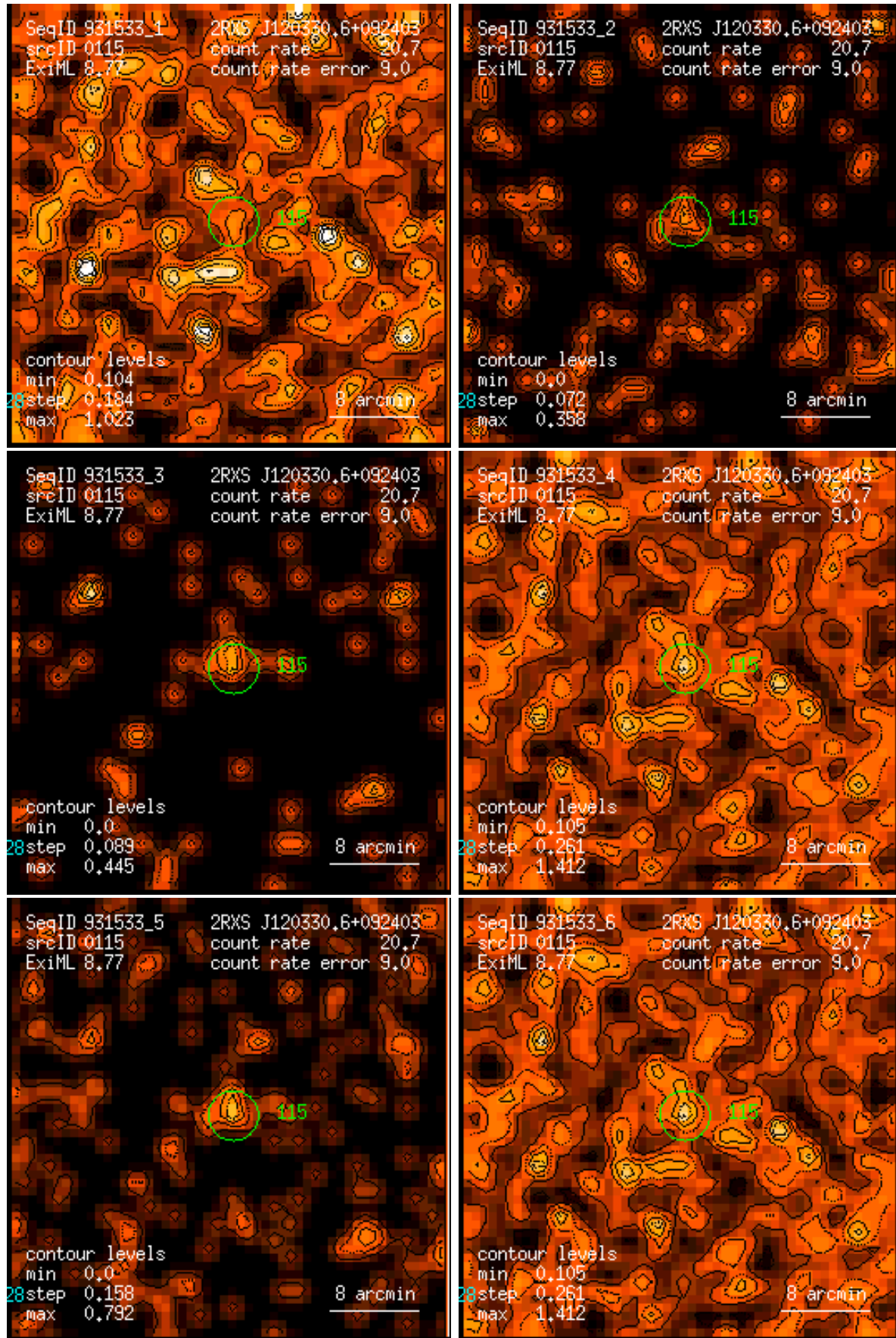
Figure 115: RASS 931533: detection 0115: band rate images, Gaussian filter: (1) PSPC channels 11 – 41, (2) 52 – 90, (3) 91 – 201, (4) 11 – 235, (5) 52 – 201, (6) 11 – 201. Broad band rates in counts/ks. Band rate contour levels in counts/ks/arcmin 2 .
