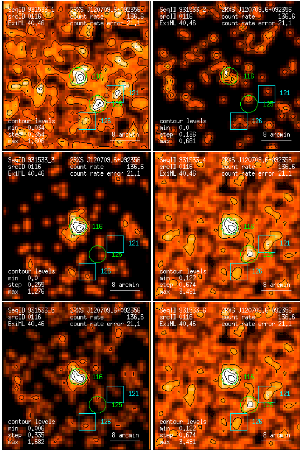
Figure 116: RASS 931533: detection 0116: band rate images, Gaussian filter: (1) PSPC channels 11 – 41, (2) 52 – 90, (3) 91 – 201, (4) 11 – 235, (5) 52 – 201, (6) 11 – 201. Broad band rates in counts/ks. Band rate contour levels in counts/ks/arcmin 2 .
