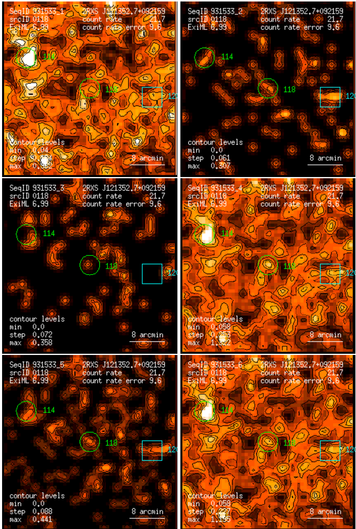
Figure 118: RASS 931533: detection 0118: band rate images, Gaussian filter: (1) PSPC channels 11 – 41, (2) 52 – 90, (3) 91 – 201, (4) 11 – 235, (5) 52 – 201, (6) 11 – 201. Broad band rates in counts/ks. Band rate contour levels in counts/ks/arcmin 2 .
