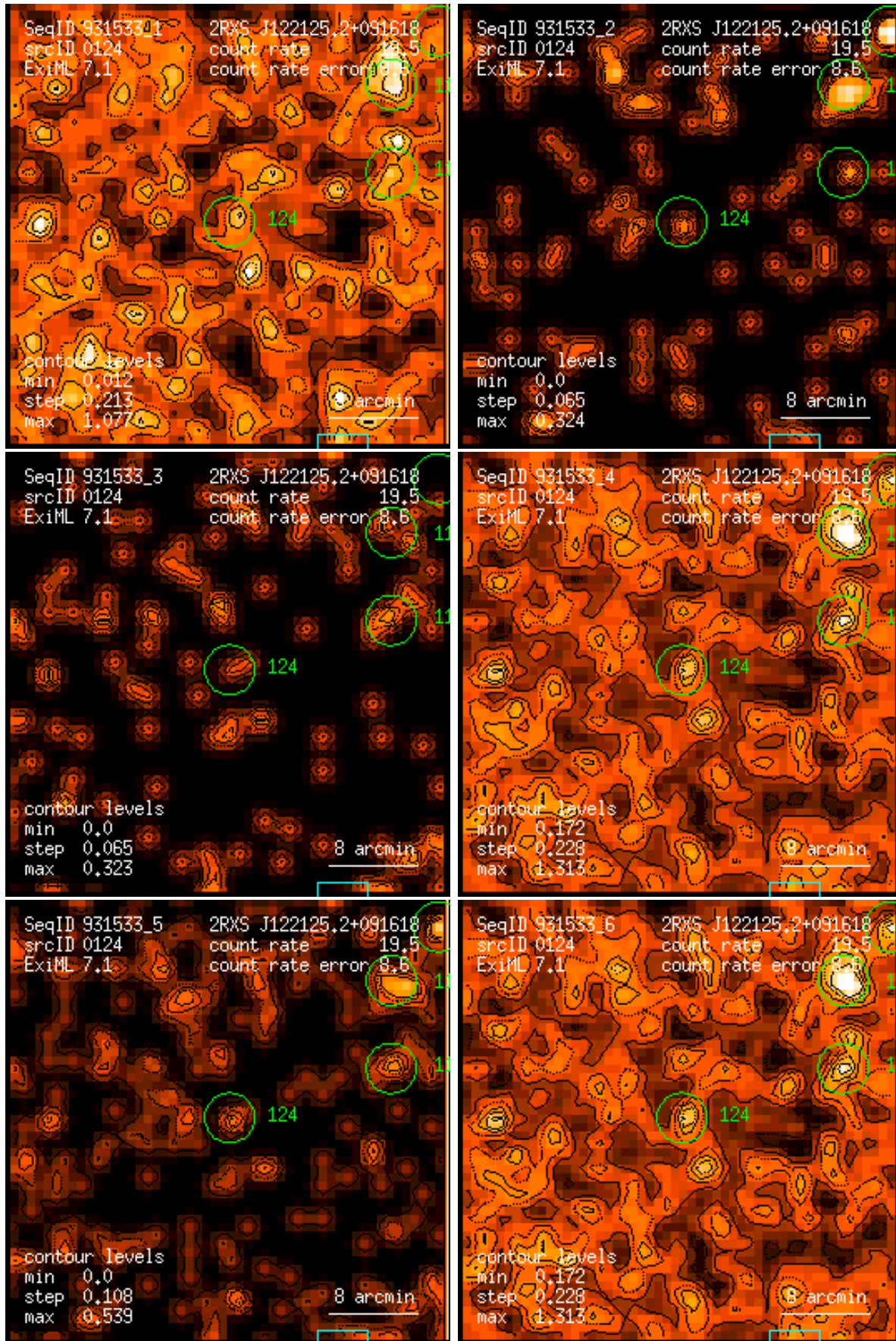
Figure 124: RASS 931533: detection 0124: band rate images, Gaussian filter: (1) PSPC channels 11 – 41, (2) 52 – 90, (3) 91 – 201, (4) 11 – 235, (5) 52 – 201, (6) 11 – 201. Broad band rates in counts/ks. Band rate contour levels in counts/ks/arcmin 2 .
