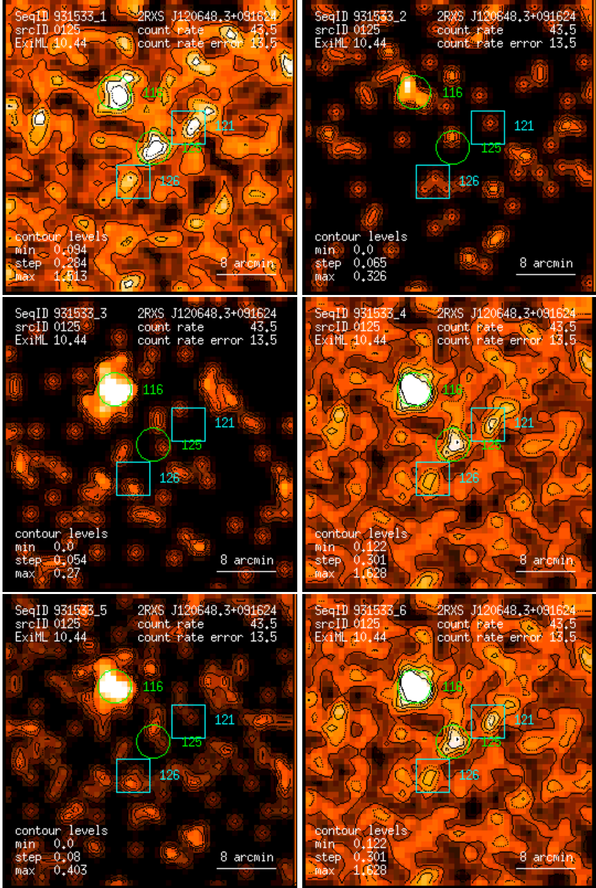
Figure 125: RASS 931533: detection 0125: band rate images, Gaussian filter: (1) PSPC channels 11 – 41, (2) 52 – 90, (3) 91 – 201, (4) 11 – 235, (5) 52 – 201, (6) 11 – 201. Broad band rates in counts/ks. Band rate contour levels in counts/ks/arcmin 2 .
