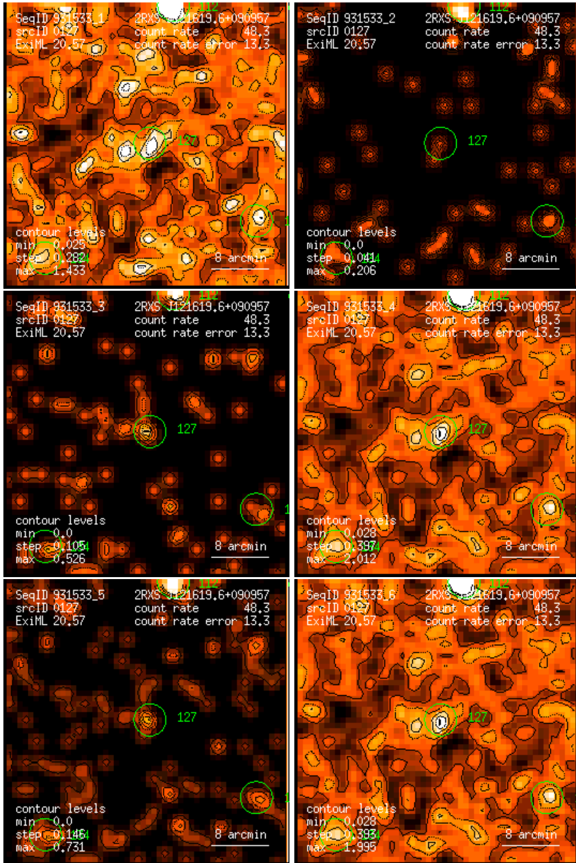
Figure 127: RASS 931533: detection 0127: band rate images, Gaussian filter: (1) PSPC channels 11 – 41, (2) 52 – 90, (3) 91 – 201, (4) 11 – 235, (5) 52 – 201, (6) 11 – 201. Broad band rates in counts/ks. Band rate contour levels in counts/ks/arcmin 2 .
