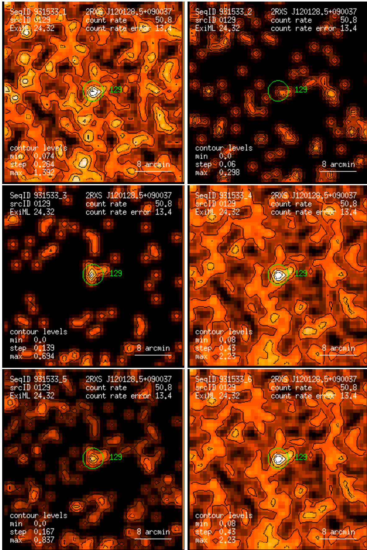
Figure 129: RASS 931533: detection 0129: band rate images, Gaussian filter: (1) PSPC channels 11 – 41, (2) 52 – 90, (3) 91 – 201, (4) 11 – 235, (5) 52 – 201, (6) 11 – 201. Broad band rates in counts/ks. Band rate contour levels in counts/ks/arcmin 2 .
