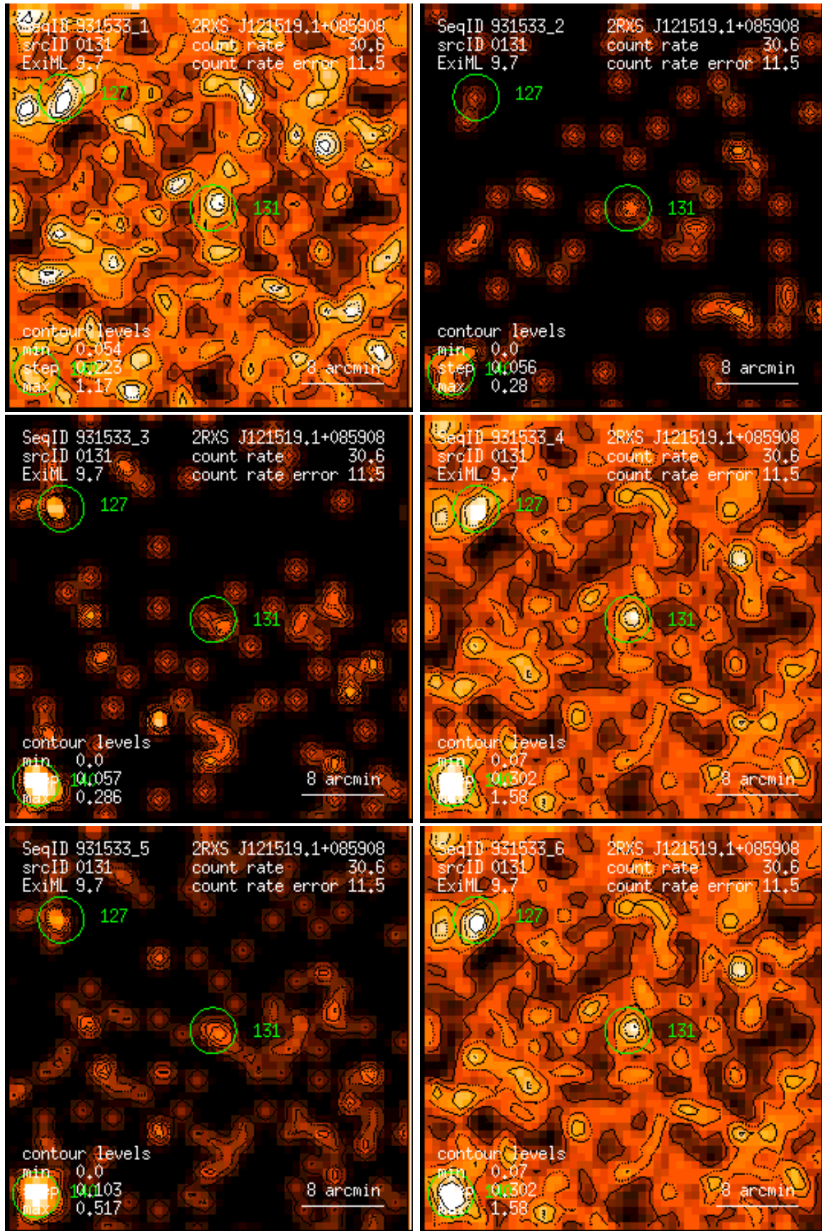
Figure 131: RASS 931533: detection 0131: band rate images, Gaussian filter: (1) PSPC channels 11 – 41, (2) 52 – 90, (3) 91 – 201, (4) 11 – 235, (5) 52 – 201, (6) 11 – 201. Broad band rates in counts/ks. Band rate contour levels in counts/ks/arcmin 2 .
