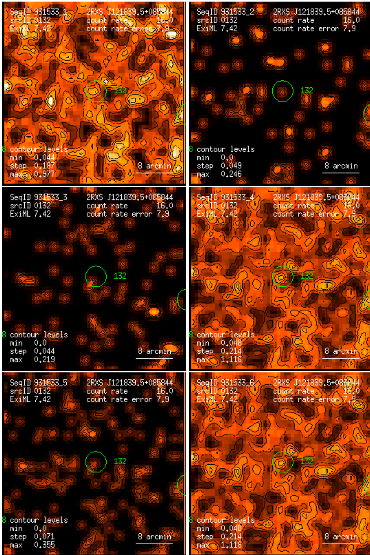
Figure 132: RASS 931533: detection 0132: band rate images, Gaussian filter: (1) PSPC channels 11 – 41, (2) 52 – 90, (3) 91 – 201, (4) 11 – 235, (5) 52 – 201, (6) 11 – 201. Broad band rates in counts/ks. Band rate contour levels in counts/ks/arcmin 2 .
