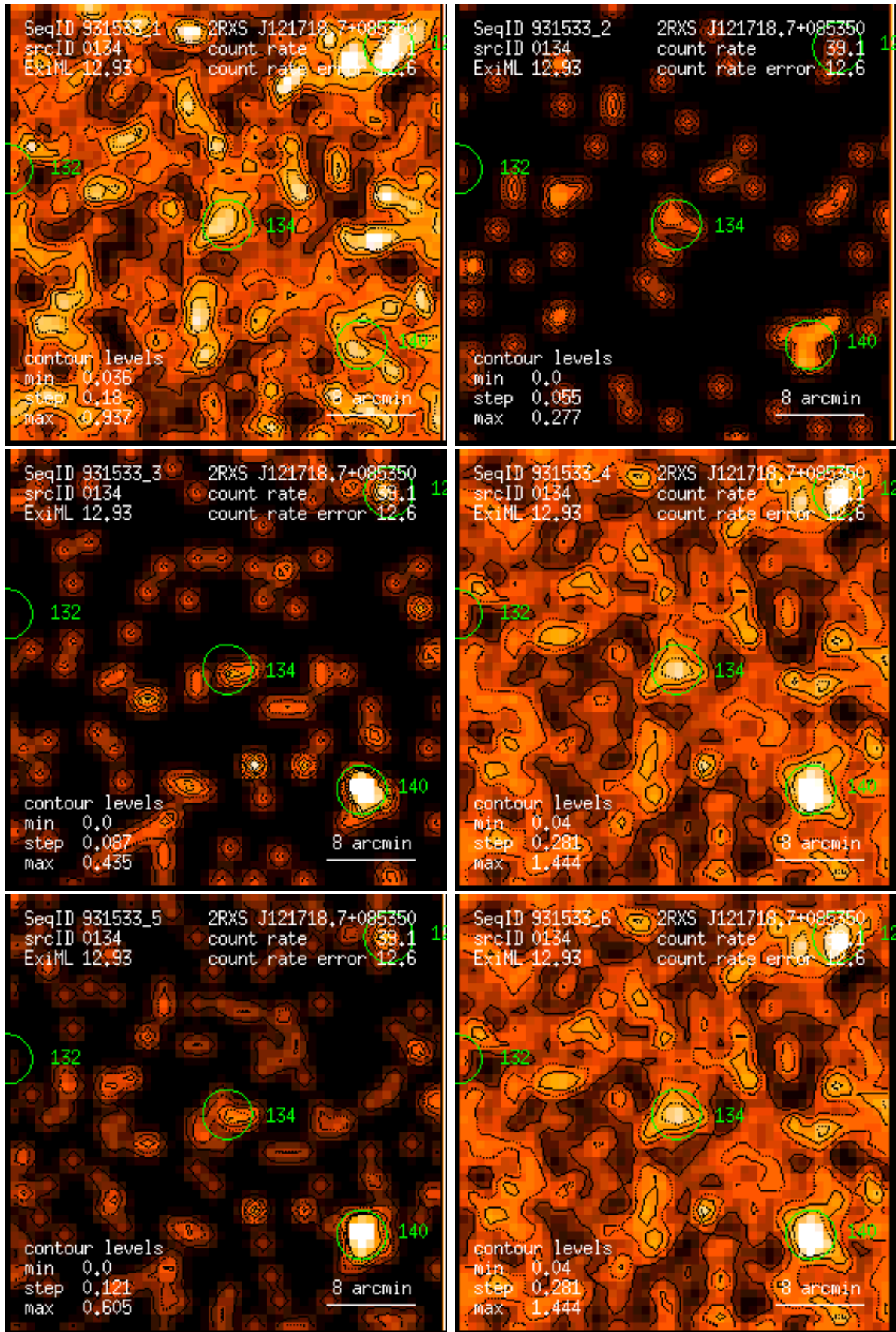
Figure 134: RASS 931533: detection 0134: band rate images, Gaussian filter: (1) PSPC channels 11 – 41, (2) 52 – 90, (3) 91 – 201, (4) 11 – 235, (5) 52 – 201, (6) 11 – 201. Broad band rates in counts/ks. Band rate contour levels in counts/ks/arcmin 2 .
