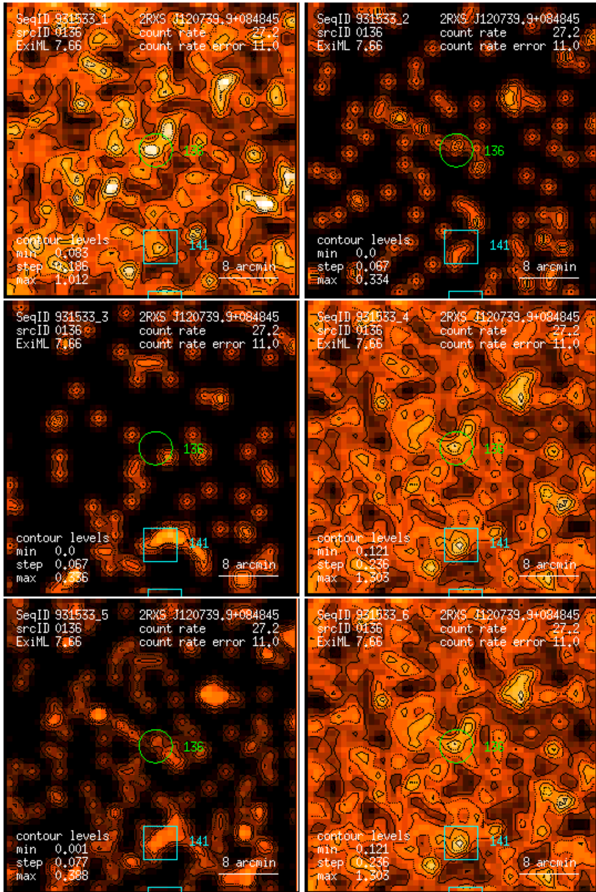
Figure 136: RASS 931533: detection 0136: band rate images, Gaussian filter: (1) PSPC channels 11 – 41, (2) 52 – 90, (3) 91 – 201, (4) 11 – 235, (5) 52 – 201, (6) 11 – 201. Broad band rates in counts/ks. Band rate contour levels in counts/ks/arcmin 2 .
