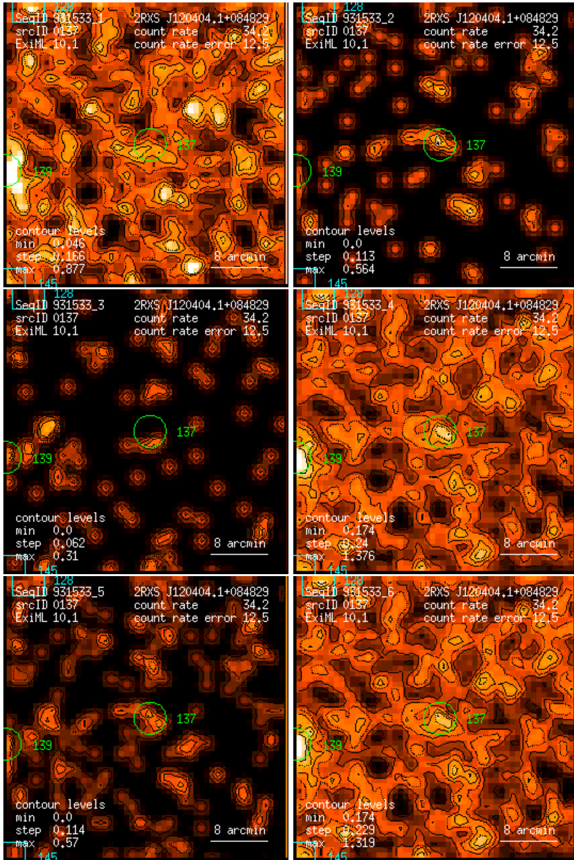
Figure 137: RASS 931533: detection 0137: band rate images, Gaussian filter: (1) PSPC channels 11 – 41, (2) 52 – 90, (3) 91 – 201, (4) 11 – 235, (5) 52 – 201, (6) 11 – 201. Broad band rates in counts/ks. Band rate contour levels in counts/ks/arcmin 2 .
