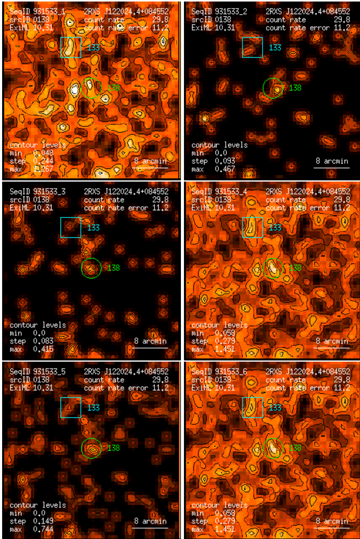
Figure 138: RASS 931533: detection 0138: band rate images, Gaussian filter: (1) PSPC channels 11 – 41, (2) 52 – 90, (3) 91 – 201, (4) 11 – 235, (5) 52 – 201, (6) 11 – 201. Broad band rates in counts/ks. Band rate contour levels in counts/ks/arcmin 2 .
