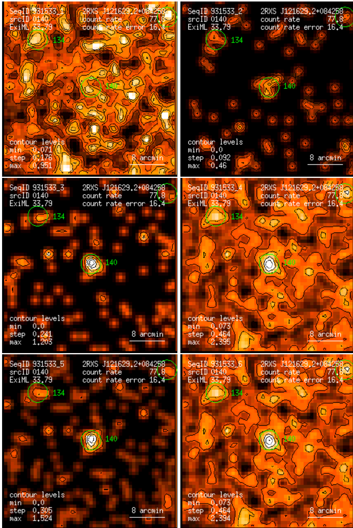
Figure 140: RASS 931533: detection 0140: band rate images, Gaussian filter: (1) PSPC channels 11 – 41, (2) 52 – 90, (3) 91 – 201, (4) 11 – 235, (5) 52 – 201, (6) 11 – 201. Broad band rates in counts/ks. Band rate contour levels in counts/ks/arcmin 2 .
