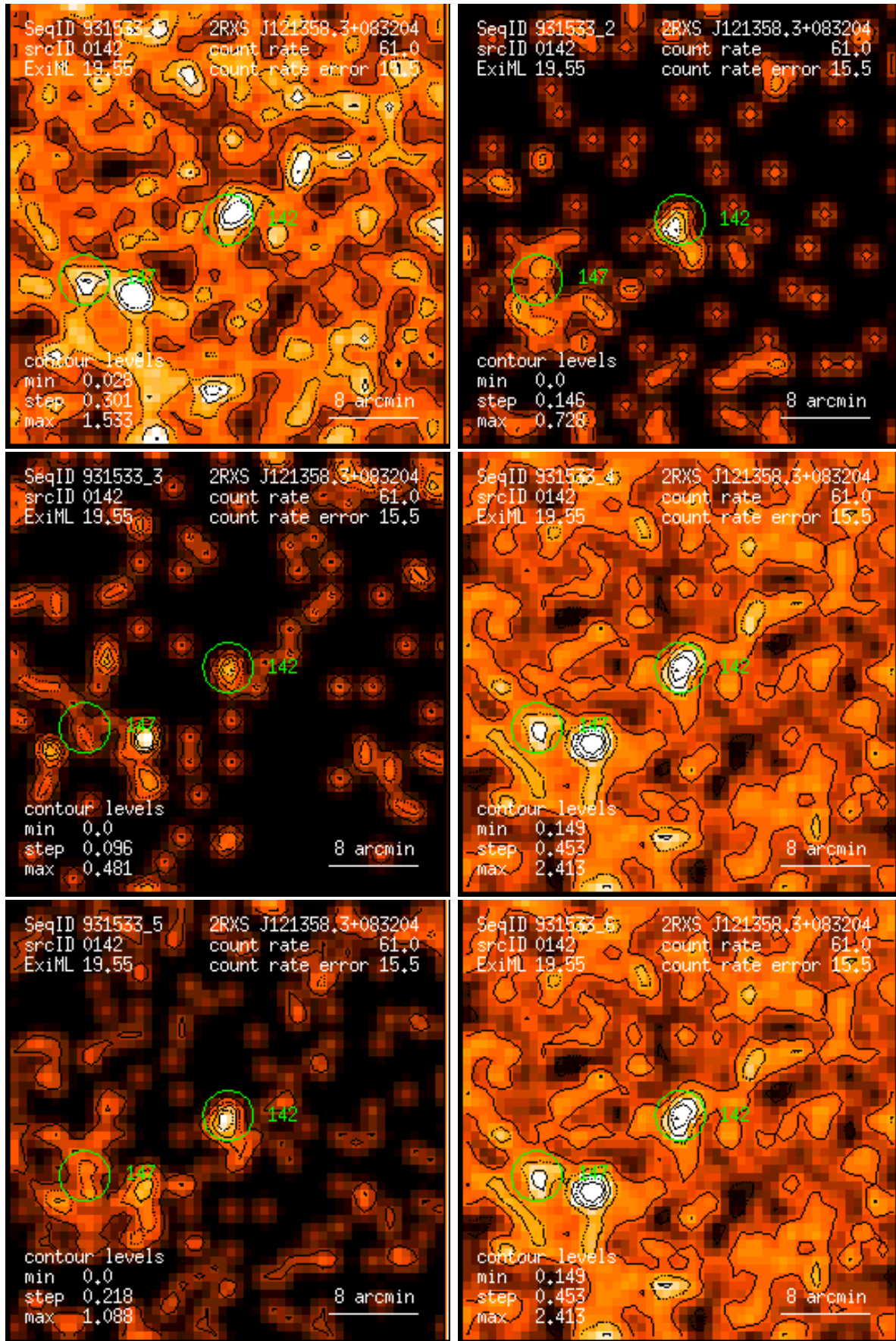
Figure 142: RASS 931533: detection 0142: band rate images, Gaussian filter: (1) PSPC channels 11 – 41, (2) 52 – 90, (3) 91 – 201, (4) 11 – 235, (5) 52 – 201, (6) 11 – 201. Broad band rates in counts/ks. Band rate contour levels in counts/ks/arcmin 2 .
